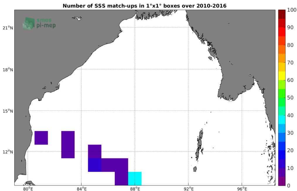
Figure 4: Number of SSS match-ups between TSG (LEGOS-DM) SSS and the SMOS SSS L2Q v321 - 0.25 Deg (CATDS-CPDC) SSS product for the Bay of Bengal Pi-MEP region over 1^\circ \times 1^\circ boxes and for the full satellite product period.
