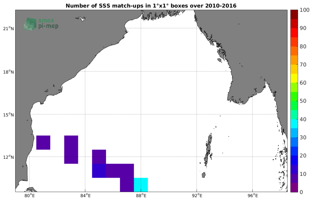
Figure 4: Number of SSS match-ups between TSG (LEGOS-DM) SSS and the SMOS SSS L2Q v321 - 0.25 Deg (CATDS-CPDC) SSS product for the Bay of Bengal Pi-MEP region over 1°x1° boxes and for the full satellite product period.
