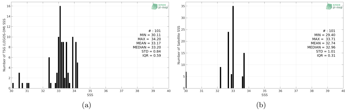
Figure 2: Histograms of SSS from TSG (LEGOS-DM) (a) and SMOS SSS L2Q v321 - 0.25 Deg (CATDS-CPDC) (b) considering all match-up pairs per bins of 0.1 over the Bay of Bengal Pi-MEP region and for the full satellite product period.
