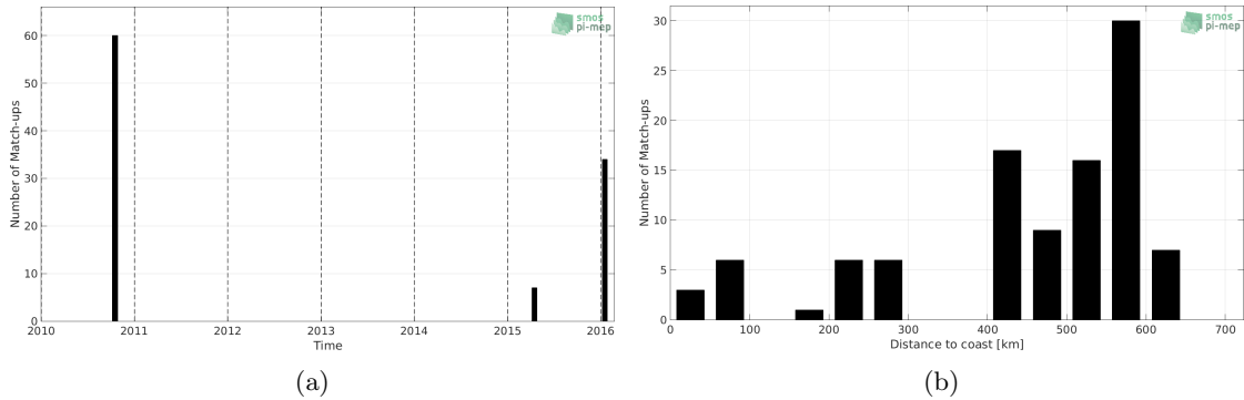
Figure 1: Number of match-ups between TSG (LEGOS-DM) and SMOS SSS L2Q v321 - 0.25 Deg (CATDS-CPDC) SSS as a function of time (a) and as function of the distance to coast (b) over the Bay of Bengal Pi-MEP region and for the full satellite product period.
