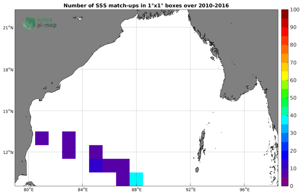
Figure 4: Number of SSS match-ups between TSG-LEGOS-DM SSS and the SMOS L2Q v321 - 0.25 Deg (CATDS-CPDC) SSS product for the Bay of Bengal Pi-MEP region over 1°x1° boxes and for the full satellite product period.
