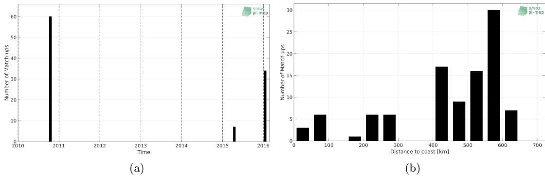
Figure 1: Number of match-ups between TSG-LEGOS-DM and SMOS L2Q v321 - 0.25 Deg (CATDS-CPDC) SSS as a function of time (a) and as function of the distance to coast (b) over the Bay of Bengal Pi-MEP region and for the full satellite product period.
