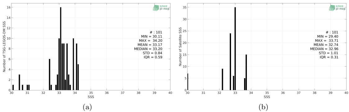
Figure 2: Histograms of SSS from TSG-LEGOS-DM (a) and SMOS L2Q v321 - 0.25 Deg (CATDS-CPDC) (b) considering all match-up pairs per bins of 0.1 over the Bay of Bengal Pi-MEP region and for the full satellite product period.
