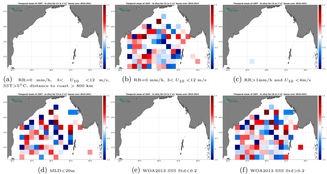
Figure 12: Temporal mean gridded over spatial boxes of size 1°x1° of \Delta SSS (SMOS SSS L2Q v321 - 0.25 Deg (CATDS-CPDC) - Argo) for 6 different subdatasets corresponding to:RR=0 mm/h, 3 < U_{10} < 12 m/s, SST>5°C, distance to coast > 800 km (a), RR=0 mm/h, 3 < U_{10} < 12 m/s (b), RR>1mm/h and U_{10} < 4 m/s (c),MLD<20m (d),WOA2013 SSS Std<0.2 (e),WOA2013 SSS Std>0.2 (f).
