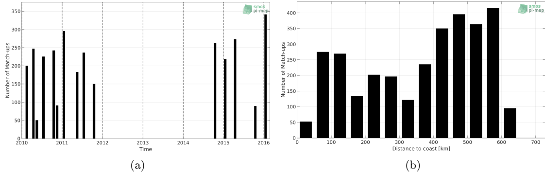
Figure 1: Number of match-ups between TSG-LEGOS-DM and SMOS L3 v317 - Monthly - 25 km (CATDS-CPDC) SSS as a function of time (a) and as function of the distance to coast (b) over the Bay of Bengal Pi-MEP region and for the full satellite product period.
