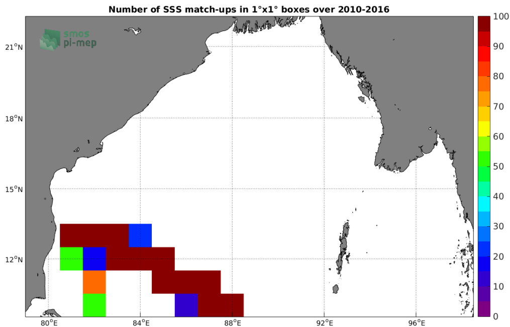
Figure 4: Number of SSS match-ups between TSG-LEGOS-DM SSS and the SMOS L3 v317 - Monthly - 25 km (CATDS-CPDC) SSS product for the Bay of Bengal Pi-MEP region over 1°x1° boxes and for the full satellite product period.
