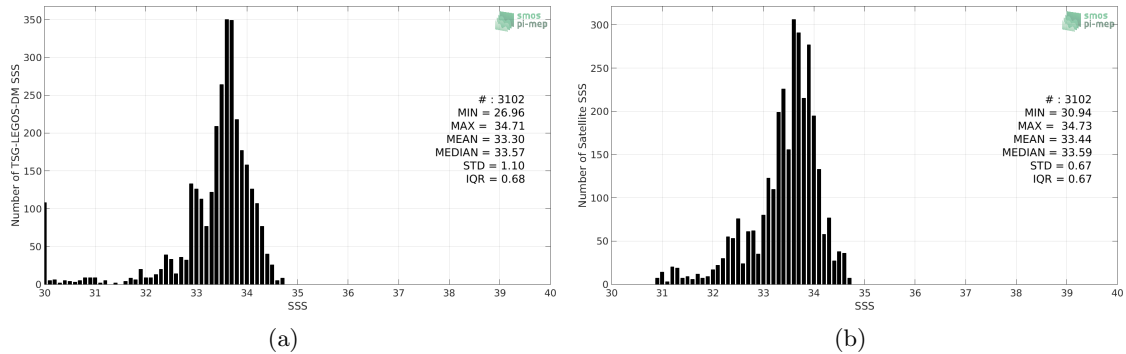
Figure 2: Histograms of SSS from TSG-LEGOS-DM (a) and SMOS L3 v317 - Monthly - 25 km (CATDS-CPDC) (b) considering all match-up pairs per bins of 0.1 over the Bay of Bengal Pi-MEP region and for the full satellite product period.
