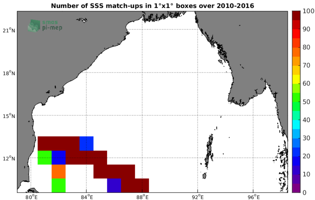
Figure 4: Number of SSS match-ups between TSG-LEGOS-DM SSS and the SMOS-L3-CATDS-CPDC-V317-MONTHLY-25KM SSS product for the Bay of Bengal Pi-MEP region over 1^\circ \times 1^\circ boxes and for the full satellite product period.
