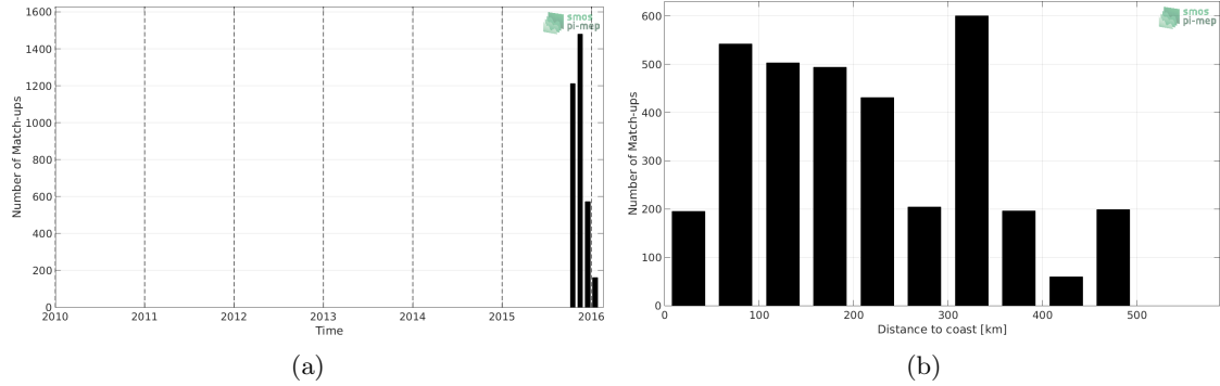
Figure 1: Number of match-ups between Surface drifters and SMOS-L3-CATDS-CPDC-V317-MONTHLY-25KM SSS as a function of time (a) and as function of the distance to coast (b) over the Bay of Bengal Pi-MEP region and for the full satellite product period.
