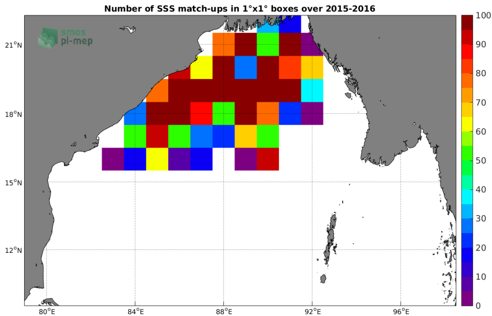
Figure 3: Number of SSS match-ups between Surface drifters SSS and the SMOS-L3-CATDS-CPDC-V317-MONTHLY-25KM SSS product for the Bay of Bengal Pi-MEP region over 1^\circ \times 1^\circ boxes and for the full satellite product period.
