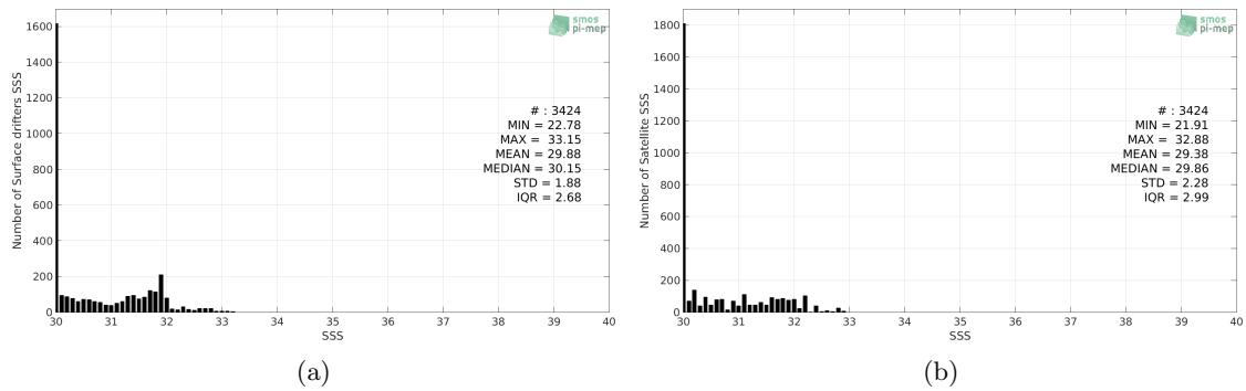
Figure 2: Histograms of SSS from Surface drifters (a) and SMOS-L3-CATDS-CPDC-V317-MONTHLY-25KM (b) considering all match-up pairs per bins of 0.1 over the Bay of Bengal Pi-MEP region and for the full satellite product period.
