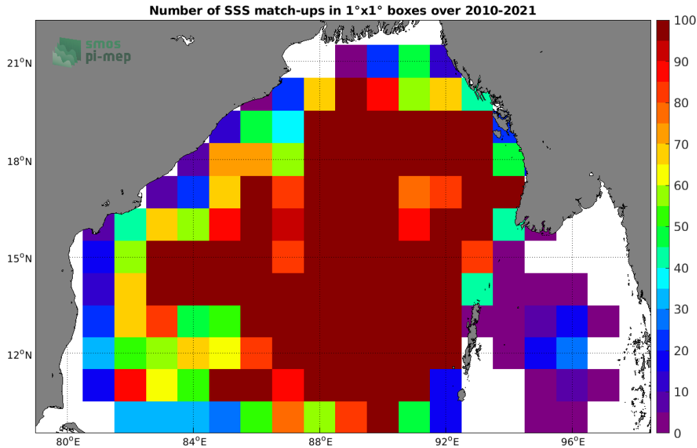
Figure 4: Number of SSS match-ups between Argo SSS and the SMOS SSS L3 v317 - Monthly - 25 km (CATDS-CPDC) SSS product for the Bay of Bengal Pi-MEP region over 1^\circ \times 1^\circ boxes and for the full satellite product period.
