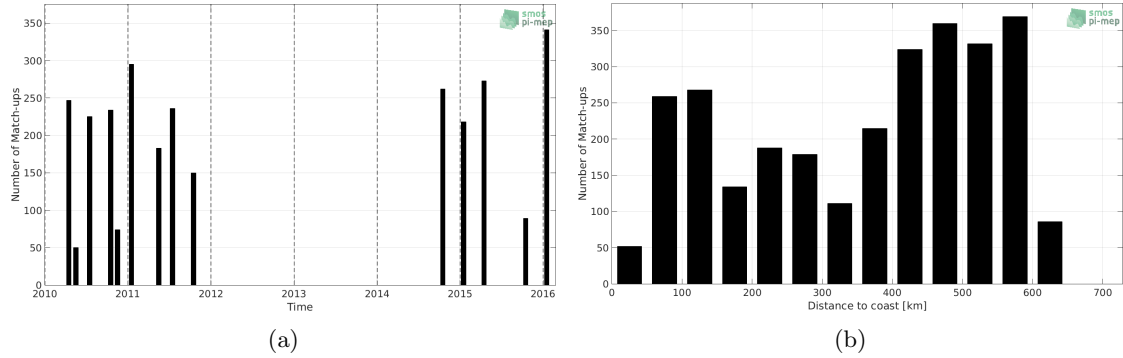
Figure 1: Number of match-ups between TSG (LEGOS-DM) and SMOS SSS L3 v317 - 10 Days - 25 km (CATDS-CPDC) SSS as a function of time (a) and as function of the distance to coast (b) over the Bay of Bengal Pi-MEP region and for the full satellite product period.
