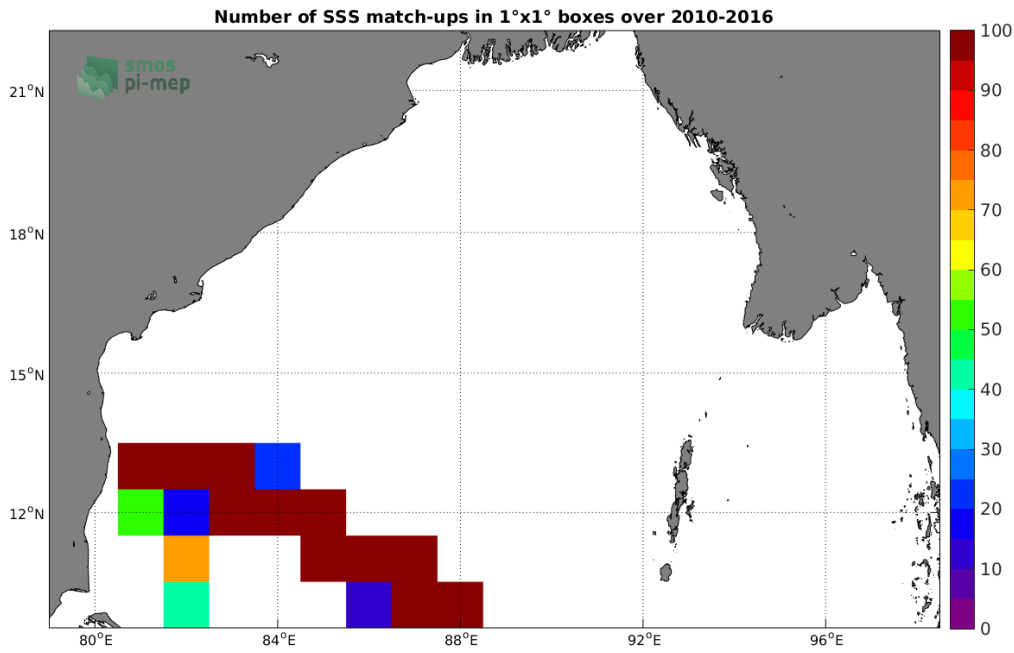
Figure 4: Number of SSS match-ups between TSG (LEGOS-DM) SSS and the SMOS SSS L3 v317 - 10 Days - 25 km (CATDS-CPDC) SSS product for the Bay of Bengal Pi-MEP region over 1^\circ \times 1^\circ boxes and for the full satellite product period.
