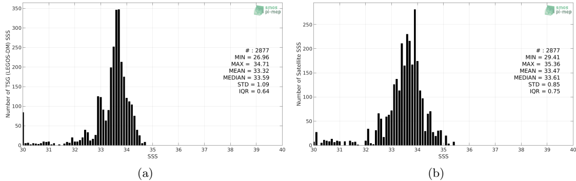
Figure 2: Histograms of SSS from TSG (LEGOS-DM) (a) and SMOS SSS L3 v317 - 10 Days - 25 km (CATDS-CPDC) (b) considering all match-up pairs per bins of 0.1 over the Bay of Bengal Pi-MEP region and for the full satellite product period.
