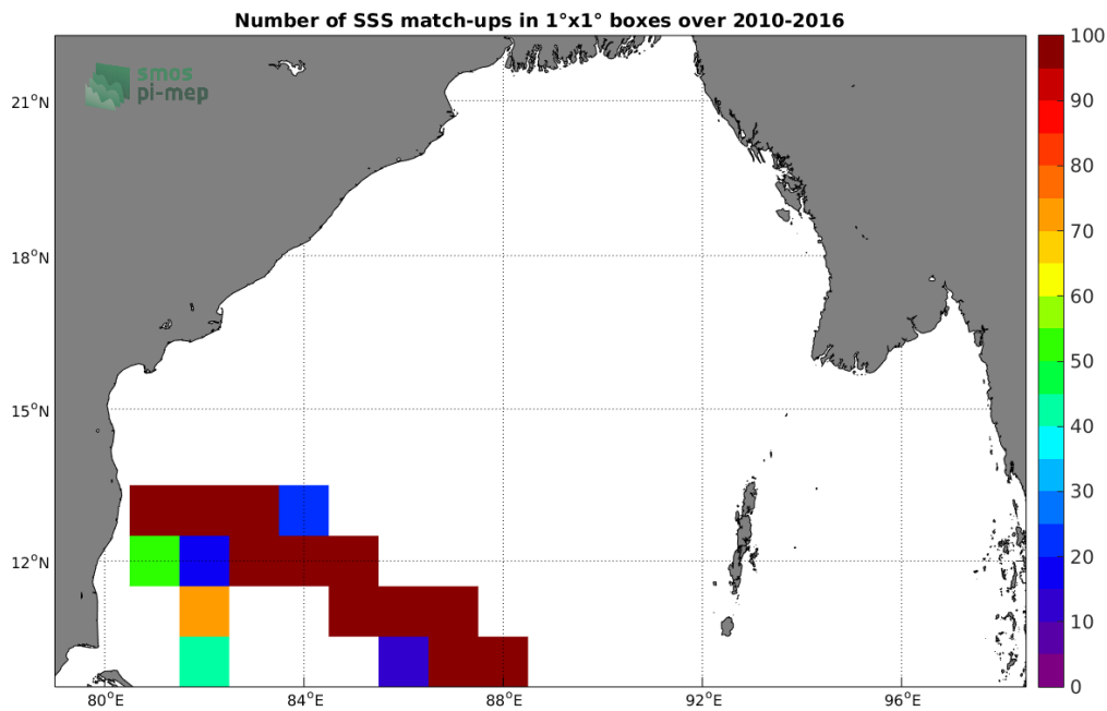
Figure 4: Number of SSS match-ups between TSG-LEGOS-DM SSS and the SMOS L3 v317 - 10 Days - 25 km (CATDS-CPDC) SSS product for the Bay of Bengal Pi-MEP region over 1^\circ \times 1^\circ boxes and for the full satellite product period.
