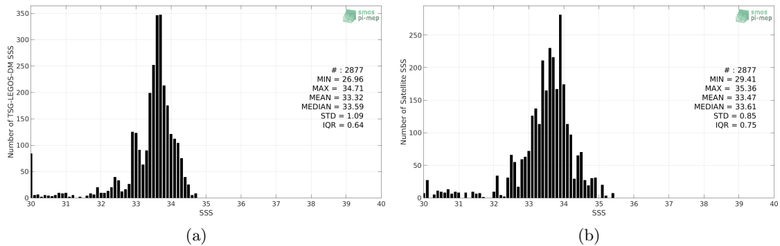
Figure 2: Histograms of SSS from TSG-LEGOS-DM (a) and SMOS L3 v317 - 10 Days - 25 km (CATDS-CPDC) (b) considering all match-up pairs per bins of 0.1 over the Bay of Bengal Pi-MEP region and for the full satellite product period.
