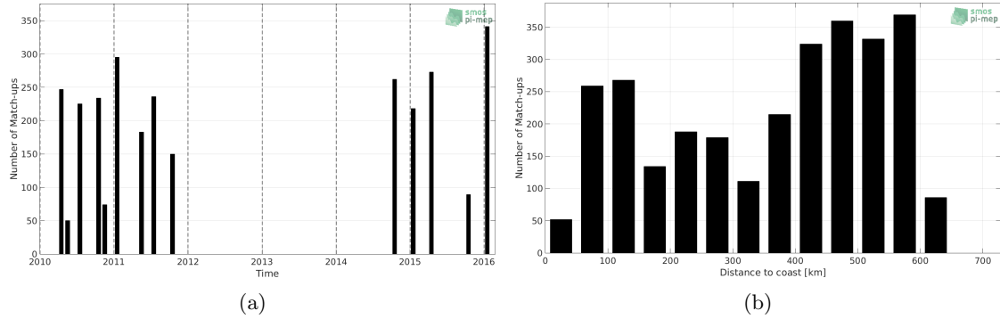
Figure 1: Number of match-ups between TSG-LEGOS-DM and SMOS L3 v317 - 10 Days - 25 km (CATDS-CPDC) SSS as a function of time (a) and as function of the distance to coast (b) over the Bay of Bengal Pi-MEP region and for the full satellite product period.
