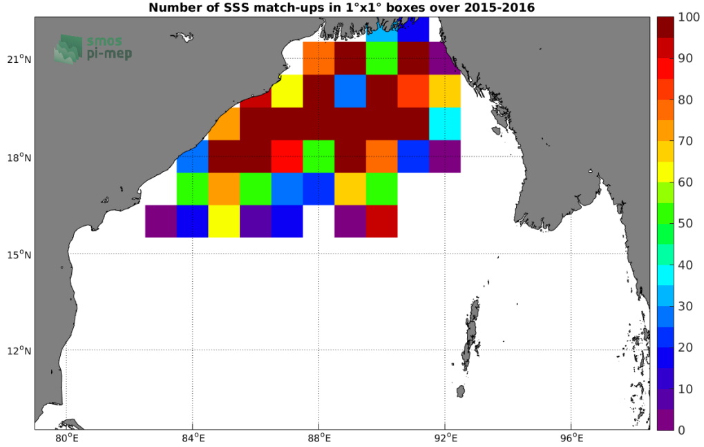
Figure 3: Number of SSS match-ups between Surface drifters SSS and the SMOS SSS L3 v317 - 10 Days - 25 km (CATDS-CPDC) SSS product for the Bay of Bengal Pi-MEP region over 1^\circ \times 1^\circ boxes and for the full satellite product period.
