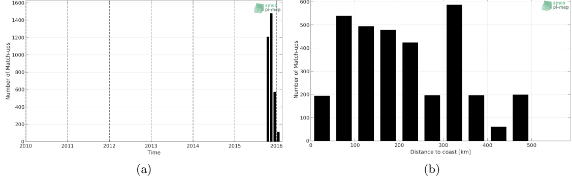
Figure 1: Number of match-ups between Surface drifters and SMOS SSS L3 v317 - 10 Days - 25 km (CATDS-CPDC) SSS as a function of time (a) and as function of the distance to coast (b) over the Bay of Bengal Pi-MEP region and for the full satellite product period.
