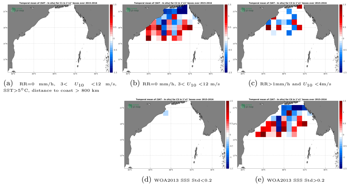
Figure 11: Temporal mean gridded over spatial boxes of size 1^\circ \times 1^\circ of \Delta SSS (SMOS SSS L3 v317 - 10 Days - 25 km (CATDS-CPDC) - Surface drifters) for 5 different subdatasets corresponding to:RR=0 mm/h, 3 < U_{10} < 12 m/s, SST >5^\circ\text{C} , distance to coast > 800 km (a), RR=0 mm/h, 3 < U_{10} < 12 m/s (b), RR >1 mm/h and U_{10} < 4 m/s (c), WOA2013 SSS Std <0.2 (d), WOA2013 SSS Std >0.2 (e).
