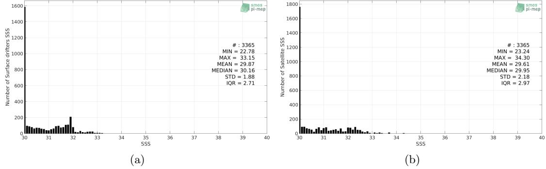
Figure 2: Histograms of SSS from Surface drifters (a) and SMOS SSS L3 v317 - 10 Days - 25 km (CATDS-CPDC) (b) considering all match-up pairs per bins of 0.1 over the Bay of Bengal Pi-MEP region and for the full satellite product period.
