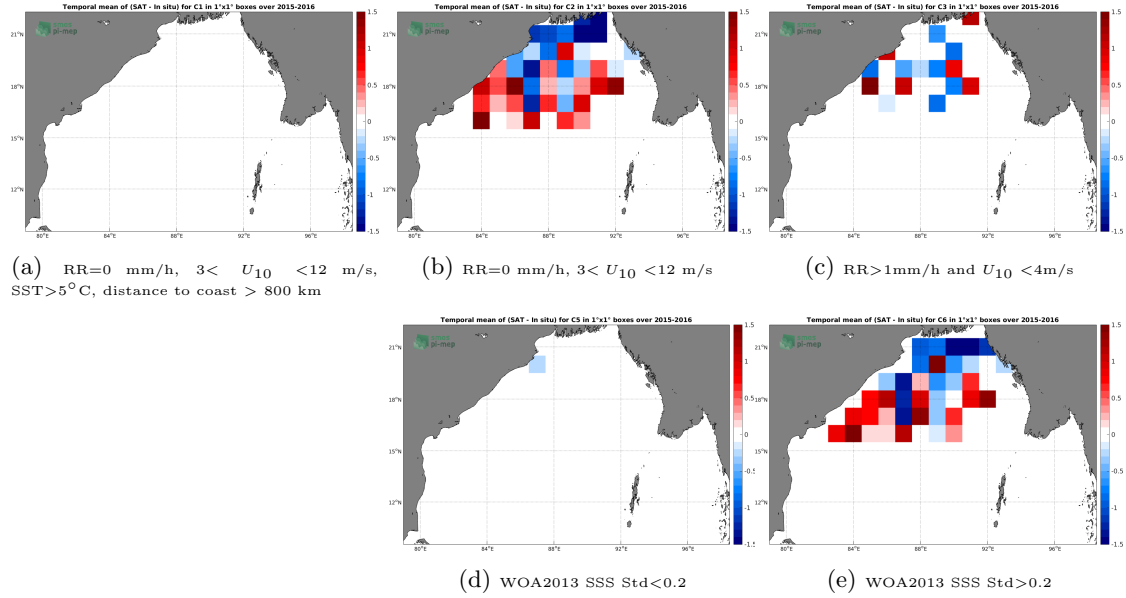
Figure 11: Temporal mean gridded over spatial boxes of size 1^\circ \times 1^\circ of \Delta SSS (SMOS L3 v317 - 10 Days - 25 km (CATDS-CPDC) - Surface drifters) for 5 different subdatasets corresponding to: RR=0 mm/h, 3 < U_{10} < 12 m/s, SST > 5^\circ C , distance to coast > 800 km (a), RR=0 mm/h, 3 < U_{10} < 12 m/s (b), RR > 1 mm/h and U_{10} < 4 m/s (c), WOA2013 SSS Std < 0.2 (d), WOA2013 SSS Std > 0.2 (e).
