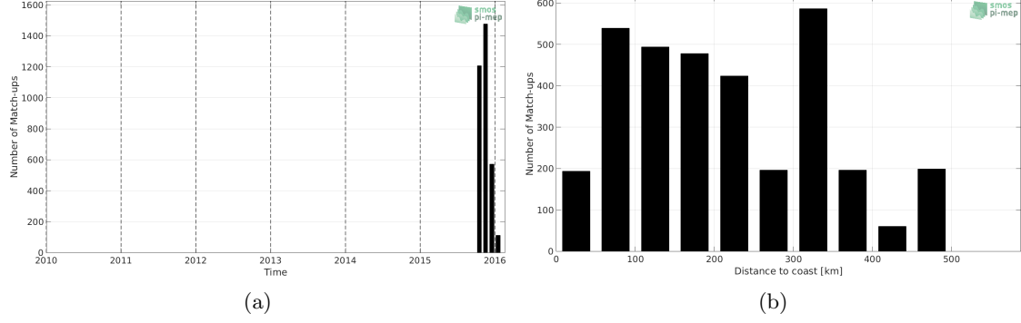
Figure 1: Number of match-ups between Surface drifters and SMOS L3 v317 - 10 Days - 25 km (CATDS-CPDC) SSS as a function of time (a) and as function of the distance to coast (b) over the Bay of Bengal Pi-MEP region and for the full satellite product period.
