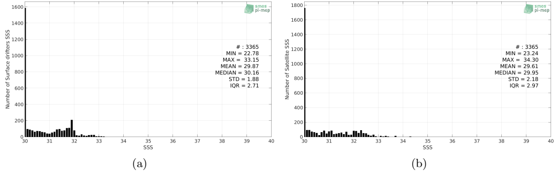
Figure 2: Histograms of SSS from Surface drifters (a) and SMOS L3 v317 - 10 Days - 25 km (CATDS-CPDC) (b) considering all match-up pairs per bins of 0.1 over the Bay of Bengal Pi-MEP region and for the full satellite product period.
