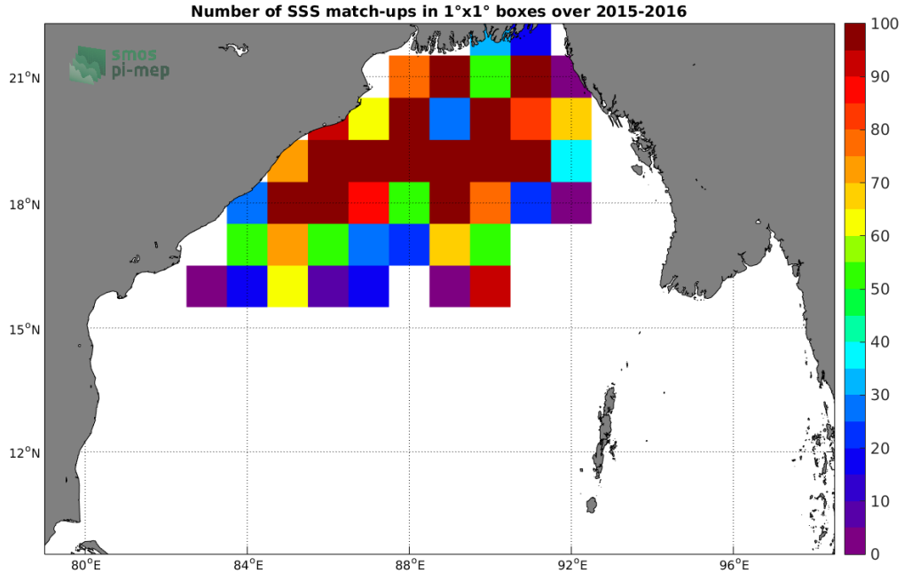
Figure 3: Number of SSS match-ups between Surface drifters SSS and the SMOS L3 v317 - 10 Days - 25 km (CATDS-CPDC) SSS product for the Bay of Bengal Pi-MEP region over 1^\circ \times 1^\circ boxes and for the full satellite product period.
