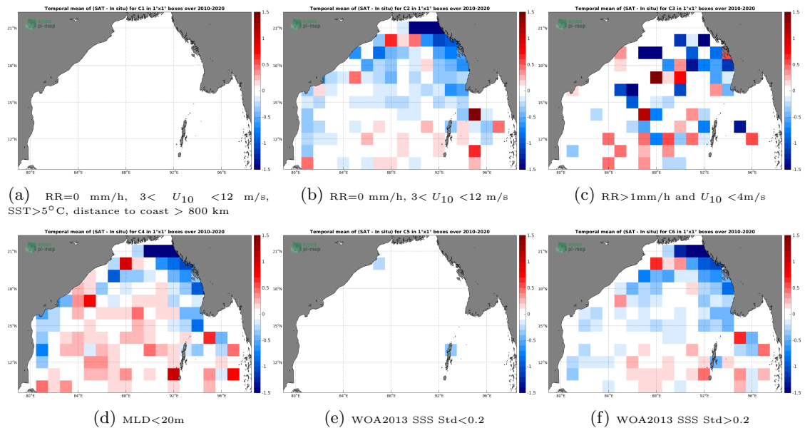
Figure 12: Temporal mean gridded over spatial boxes of size 1^\circ \times 1^\circ of \Delta SSS (SMOS SSS L3 v317 - 10 Days - 25 km (CATDS-CPDC) - Argo) for 6 different subdatasets corresponding to: RR=0 mm/h, 3 < U_{10} < 12 m/s, SST > 5^\circ C , distance to coast > 800 km (a), RR=0 mm/h, 3 < U_{10} < 12 m/s (b), RR > 1 mm/h and U_{10} < 4 m/s (c), MLD < 20 m (d), WOA2013 SSS Std < 0.2 (e), WOA2013 SSS Std > 0.2 (f).
