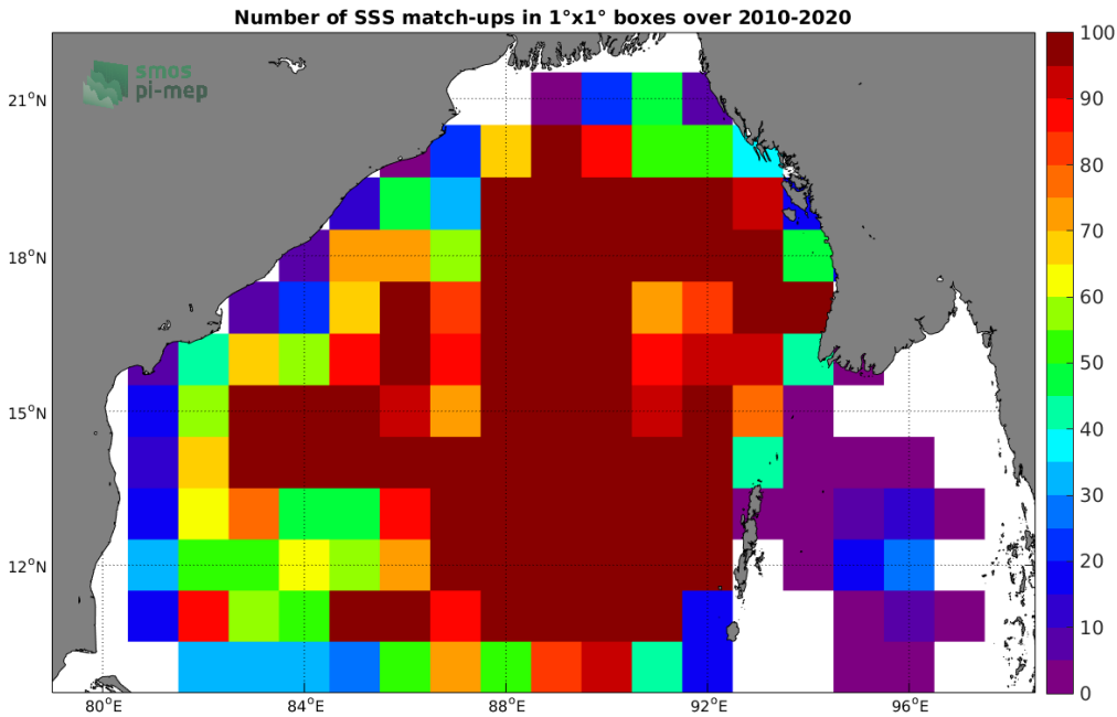
Figure 4: Number of SSS match-ups between Argo SSS and the SMOS SSS L3 v317 - 10 Days - 25 km (CATDS-CPDC) SSS product for the Bay of Bengal Pi-MEP region over 1°x1° boxes and for the full satellite product period.
