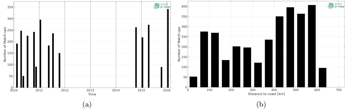
Figure 1: Number of match-ups between TSG-LEGOS-DM and SMOS-L3-CATDS-CPDC-V3-MONTHLY-25KM SSS as a function of time (a) and as function of the distance to coast (b) over the Bay of Bengal Pi-MEP region and for the full satellite product period.
