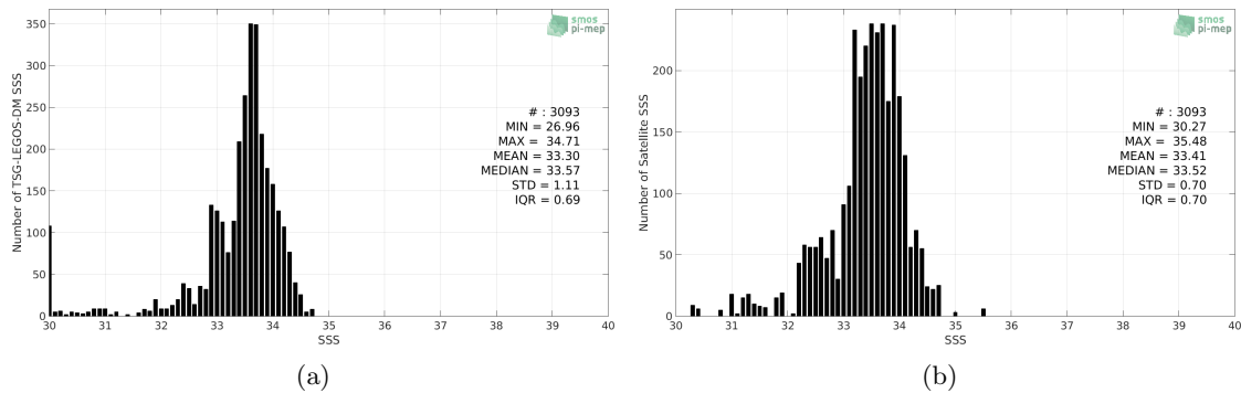
Figure 2: Histograms of SSS from TSG-LEGOS-DM (a) and SMOS-L3-CATDS-CPDC-V3-MONTHLY-25KM (b) considering all match-up pairs per bins of 0.1 over the Bay of Bengal Pi-MEP region and for the full satellite product period.
