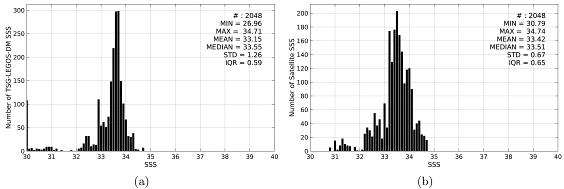
Figure 2: Histograms of SSS from TSG-LEGOS-DM (a) and SMOS-L3-CATDS-CPDC-V3-MONTHLY-25KM (b) considering all match-up pairs per bins of 0.1 over the Bay of Bengal Pi-MEP region and for the full satellite product period.
