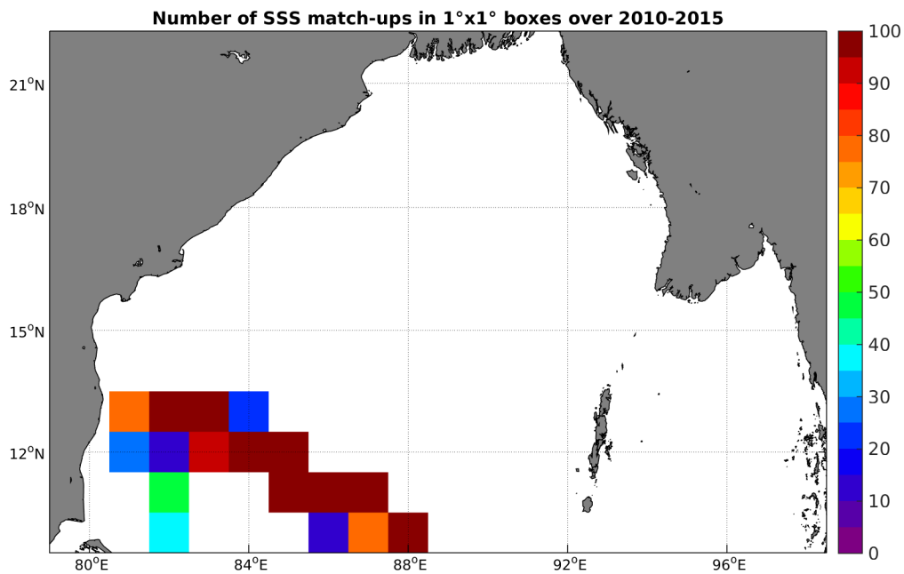
Figure 4: Number of SSS match-ups between TSG-LEGOS-DM SSS and the SMOS-L3-CATDS-CPDC-V3-MONTHLY-25KM SSS product for the Bay of Bengal Pi-MEP region over 1°x1° boxes and for the full satellite product period.
