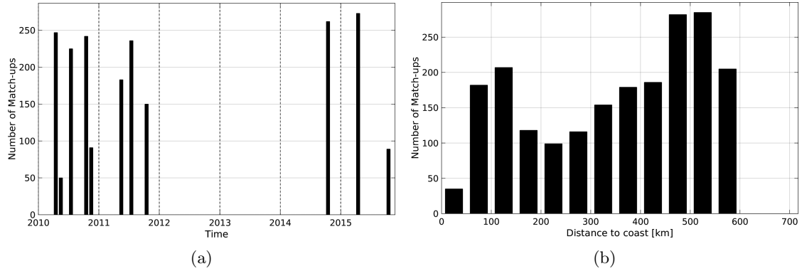
Figure 1: Number of match-ups between TSG-LEGOS-DM and SMOS-L3-CATDS-CPDC-V3-MONTHLY-25KM SSS as a function of time (a) and as function of the distance to coast (b) over the Bay of Bengal Pi-MEP region and for the full satellite product period.
