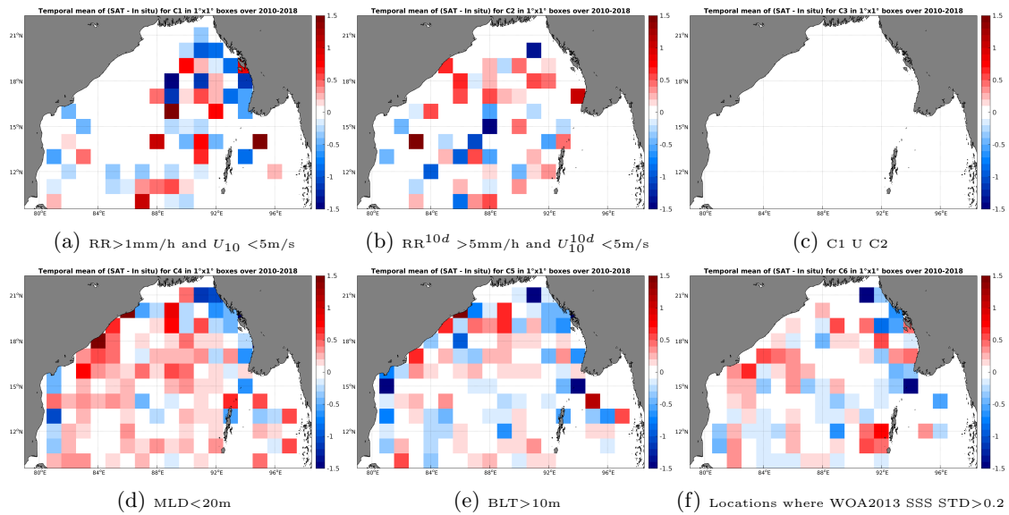
Figure 12: Temporal mean gridded over spatial boxes of size 1^\circ \times 1^\circ of \Delta SSS (SMOS-L3-CATDS-CPDC-V3-MONTHLY-25KM - Argo) for 6 different subdatasets corresponding to: RR > 1\text{mm/h} and U_{10} < 5\text{m/s} (a), RR^{10d} > 5\text{mm/h} and U_{10}^{10d} < 5\text{m/s} (b), C1 U C2 (c), MLD < 20\text{m} (d), BLT > 10\text{m} (e), Locations where WOA2013 SSS STD > 0.2 (f).
