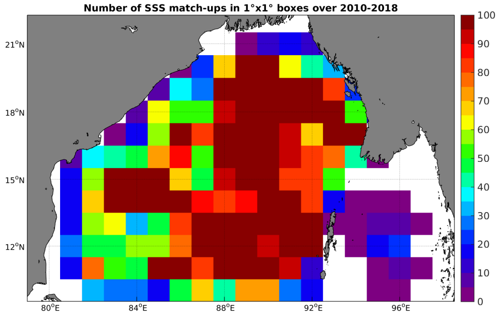
Figure 4: Number of SSS match-ups between Argo SSS and the SMOS-L3-CATDS-CPDC-V3-MONTHLY-25KM SSS product for the Bay of Bengal Pi-MEP region over 1^\circ \times 1^\circ boxes and for the full satellite product period.
