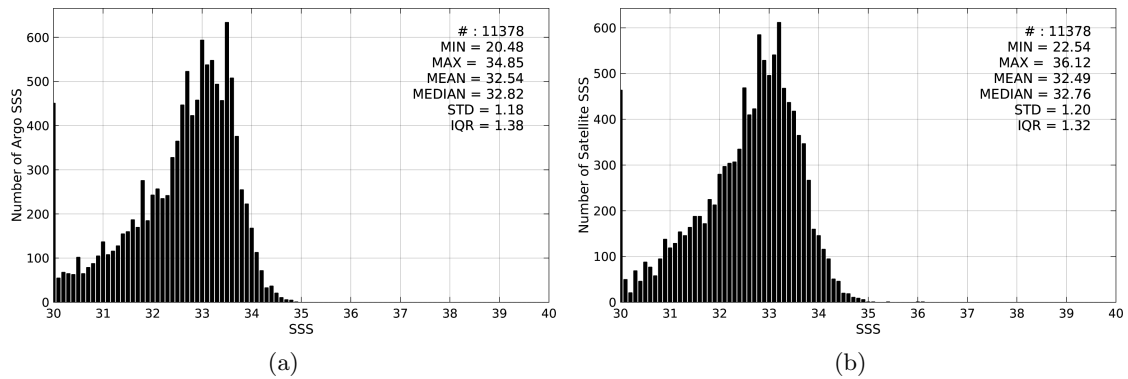
Figure 2: Histograms of SSS from Argo (a) and SMOS-L3-CATDS-CPDC-V3-MONTHLY-25KM (b) considering all match-up pairs per bins of 0.1 over the Bay of Bengal Pi-MEP region and for the full satellite product period.
