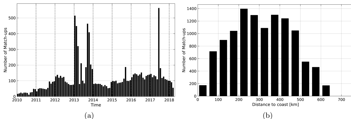
Figure 1: Number of match-ups between Argo and SMOS-L3-CATDS-CPDC-V3-MONTHLY-25KM SSS as a function of time (a) and as function of the distance to coast (b) over the Bay of Bengal Pi-MEP region and for the full satellite product period.
