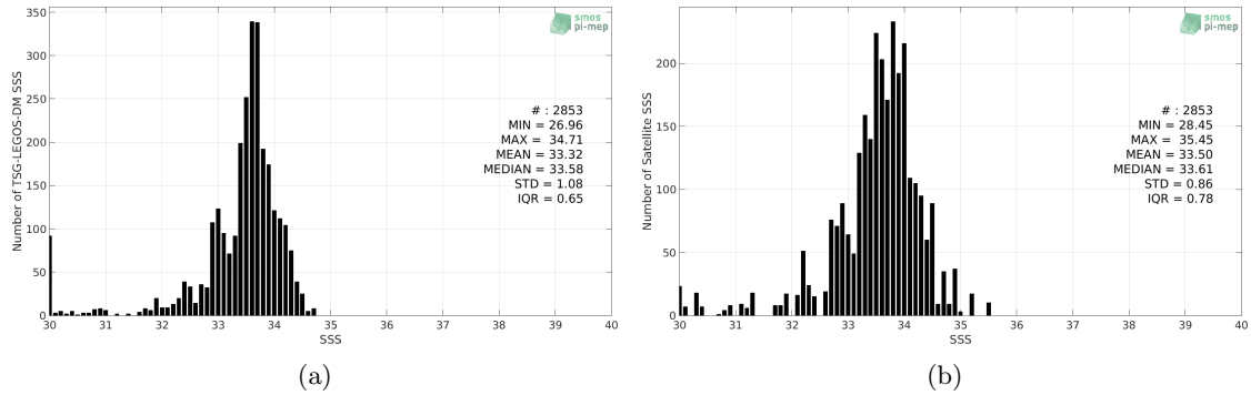
Figure 2: Histograms of SSS from TSG-LEGOS-DM (a) and SMOS-L3-CATDS-CPDC-V3-10DAYS-25KM (b) considering all match-up pairs per bins of 0.1 over the Bay of Bengal Pi-MEP region and for the full satellite product period.
