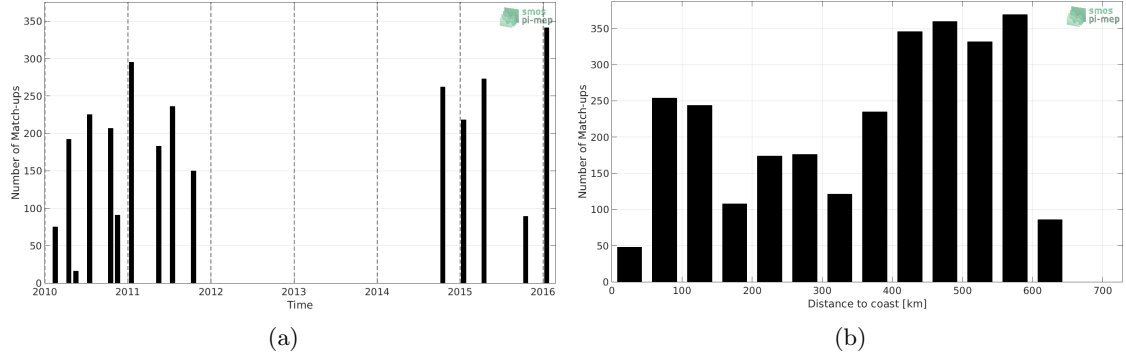
Figure 1: Number of match-ups between TSG-LEGOS-DM and SMOS-L3-CATDS-CPDC-V3-10DAYS-25KM SSS as a function of time (a) and as function of the distance to coast (b) over the Bay of Bengal Pi-MEP region and for the full satellite product period.
