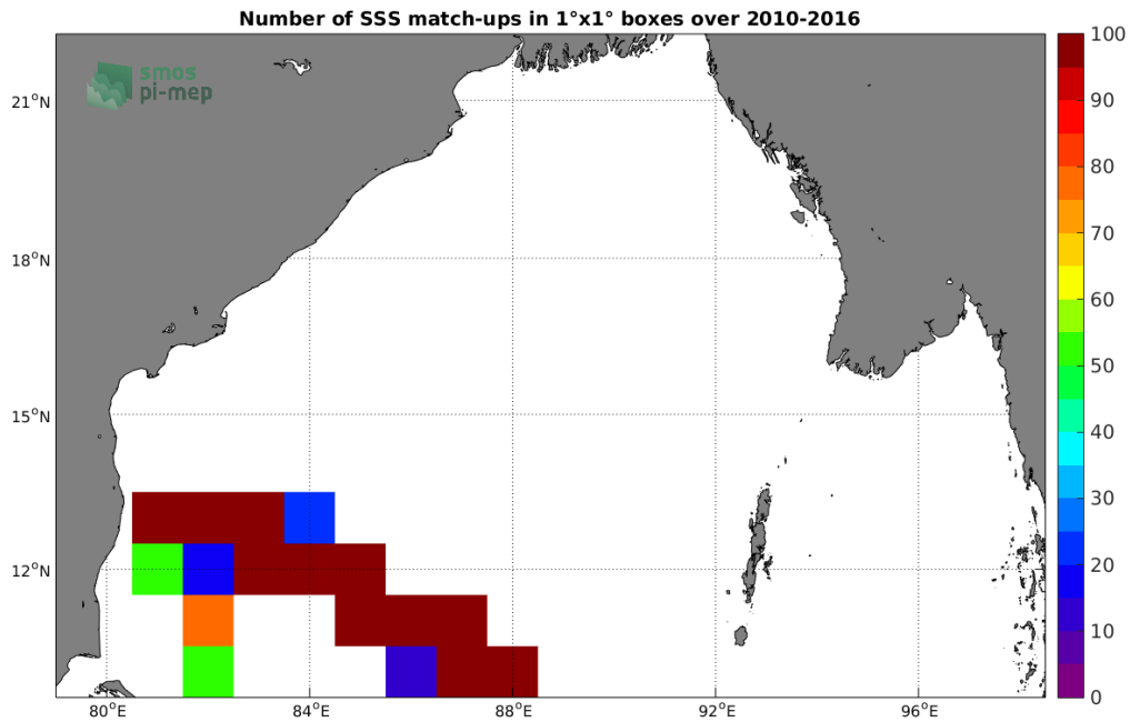
Figure 4: Number of SSS match-ups between TSG-LEGOS-DM SSS and the SMOS-L3-CATDS-CPDC-V3-10DAYS-25KM SSS product for the Bay of Bengal Pi-MEP region over 1^\circ \times 1^\circ boxes and for the full satellite product period.
