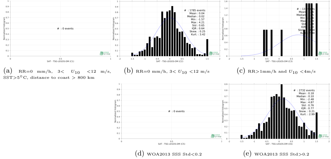
Figure 13: Normalized histogram of \Delta SSS (SMOS-L3-CATDS-CPDC-V3-10DAYS-25KM - TSG-LEGOS-DM) for 5 different subdatasets corresponding to: RR=0 mm/h, 3 < U_{10} < 12 m/s, SST > 5^\circ\text{C} , distance to coast > 800 km (a), RR=0 mm/h, 3 < U_{10} < 12 m/s (b), RR > 1 mm/h and U_{10} < 4 m/s (c), WOA2013 SSS Std < 0.2 (d), WOA2013 SSS Std > 0.2 (e).
