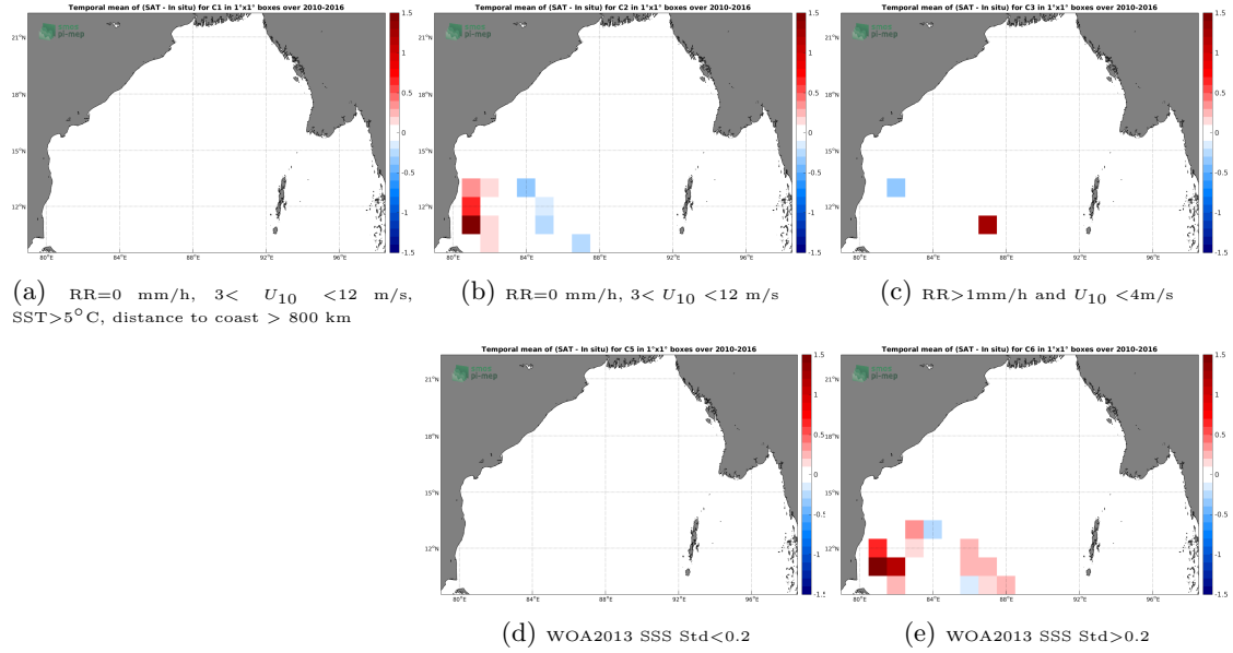
Figure 12: Temporal mean gridded over spatial boxes of size 1^\circ \times 1^\circ of \Delta SSS (SMOS-L3-CATDS-CPDC-V3-10DAYS-25KM - TSG-LEGOS-DM) for 5 different subdatasets corresponding to: RR=0 mm/h, 3 < U_{10} < 12 m/s, SST > 5^\circ C , distance to coast > 800 km (a), RR=0 mm/h, 3 < U_{10} < 12 m/s (b), RR > 1 mm/h and U_{10} < 4 m/s (c), WOA2013 SSS Std < 0.2 (d), WOA2013 SSS Std > 0.2 (e).
