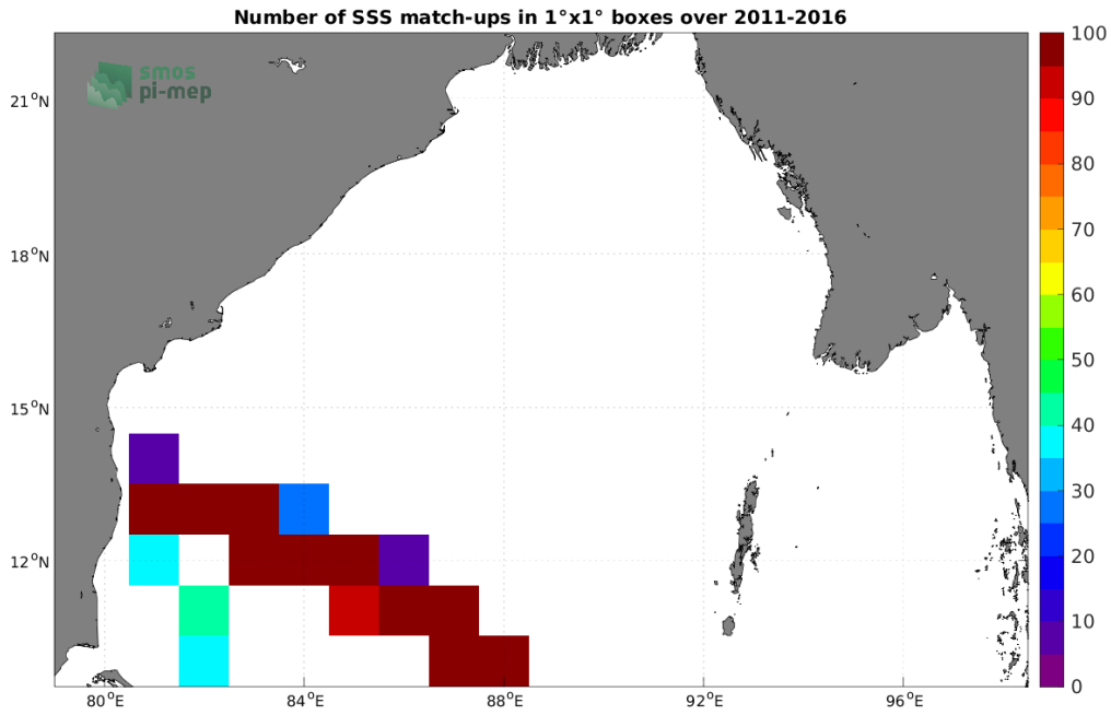
Figure 4: Number of SSS match-ups between TSG (LEGOS-DM) SSS and the SMOS SSS L3 v2 - 9-Days (BEC) SSS product for the Bay of Bengal Pi-MEP region over 1^\circ \times 1^\circ boxes and for the full satellite product period.
