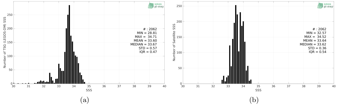
Figure 2: Histograms of SSS from TSG (LEGOS-DM) (a) and SMOS SSS L3 v2 - 9-Days (BEC) (b) considering all match-up pairs per bins of 0.1 over the Bay of Bengal Pi-MEP region and for the full satellite product period.
