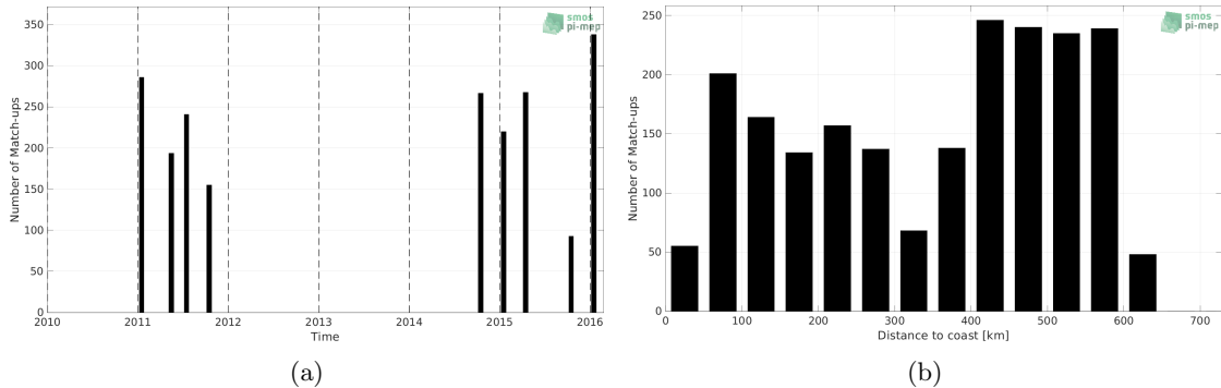
Figure 1: Number of match-ups between TSG (LEGOS-DM) and SMOS SSS L3 v2 - 9-Days (BEC) SSS as a function of time (a) and as function of the distance to coast (b) over the Bay of Bengal Pi-MEP region and for the full satellite product period.
