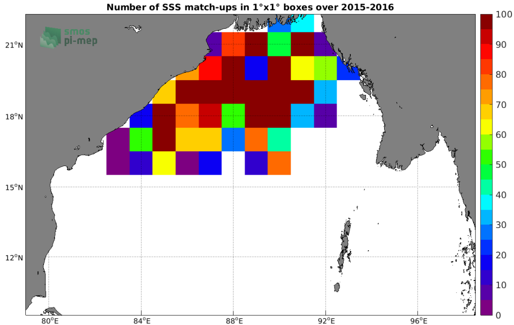
Figure 3: Number of SSS match-ups between Surface drifters SSS and the SMOS SSS L3 v2 - 9-Days (BEC) SSS product for the Bay of Bengal Pi-MEP region over 1°x1° boxes and for the full satellite product period.
