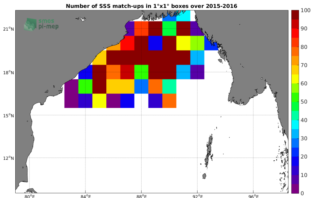
Figure 3: Number of SSS match-ups between Surface drifters SSS and the SMOS L3 v2 - 9-Days (BEC) SSS product for the Bay of Bengal Pi-MEP region over 1°x1° boxes and for the full satellite product period.
