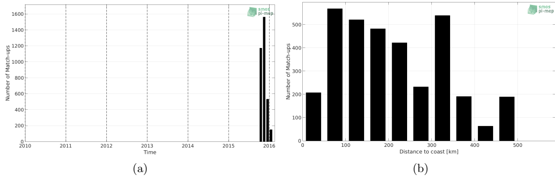
Figure 1: Number of match-ups between Surface drifters and SMOS L3 v2 - 9-Days (BEC) SSS as a function of time (a) and as function of the distance to coast (b) over the Bay of Bengal Pi-MEP region and for the full satellite product period.
