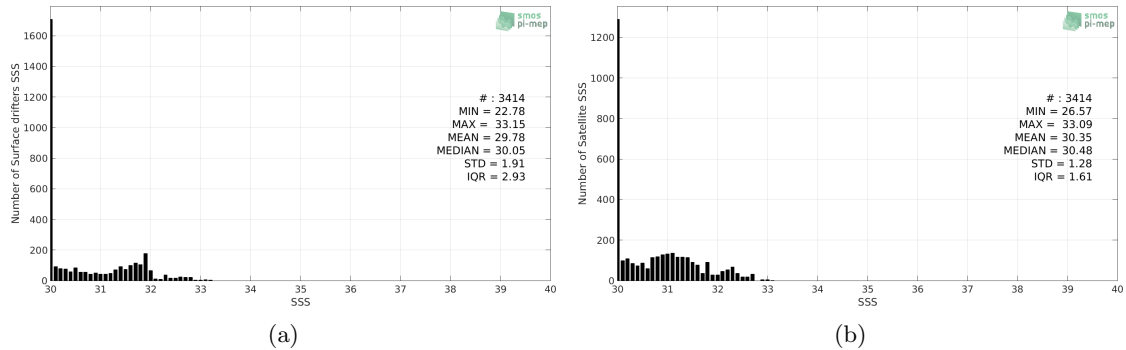
Figure 2: Histograms of SSS from Surface drifters (a) and SMOS L3 v2 - 9-Days (BEC) (b) considering all match-up pairs per bins of 0.1 over the Bay of Bengal Pi-MEP region and for the full satellite product period.
