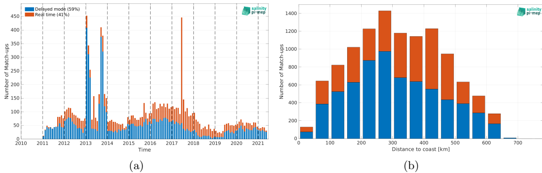
Figure 2: Number of match-ups between Argo and SMOS SSS L3 v2 - 9-Days (BEC) SSS as a function of time (a) and as function of the distance to coast (b) over the Bay of Bengal Pi-MEP region and for the full satellite product period.
