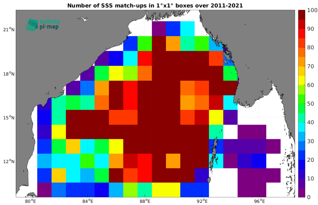
Figure 5: Number of SSS match-ups between Argo SSS and the SMOS SSS L3 v2 - 9-Days (BEC) SSS product for the Bay of Bengal Pi-MEP region over 1^{\circ} \times 1^{\circ} boxes and for the full satellite product period.
