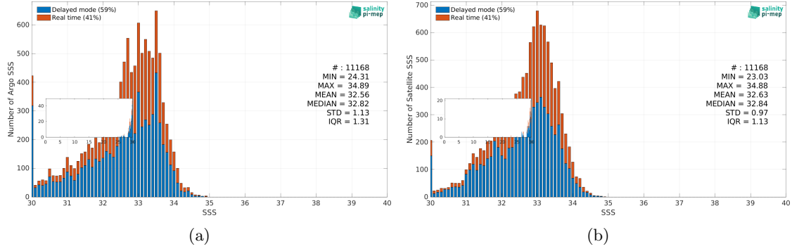
Figure 3: Histograms of SSS from Argo (a) and SMOS SSS L3 v2 - 9-Days (BEC) (b) considering all match-up pairs per bins of 0.1 over the Bay of Bengal Pi-MEP region and for the full satellite product period.
