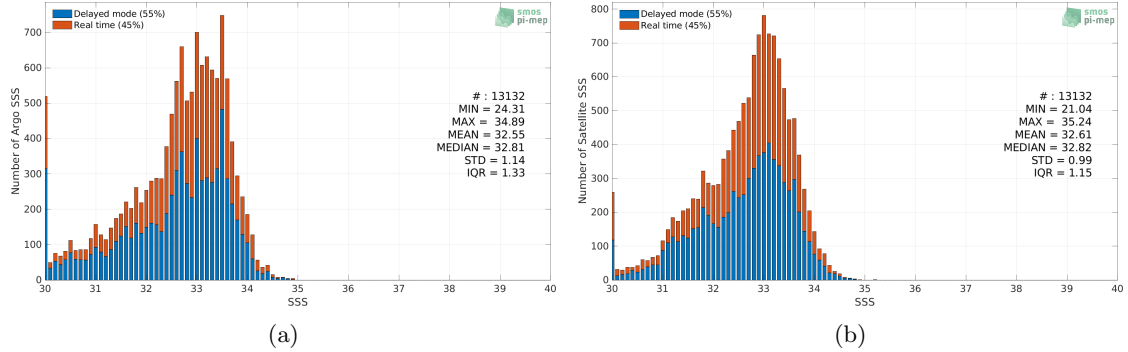
Figure 2: Histograms of SSS from Argo (a) and SMOS SSS L3 v2 - 9-Days (BEC) (b) considering all match-up pairs per bins of 0.1 over the Bay of Bengal Pi-MEP region and for the full satellite product period.
