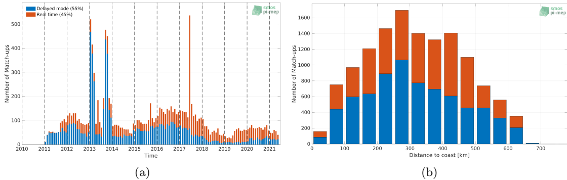
Figure 1: Number of match-ups between Argo and SMOS SSS L3 v2 - 9-Days (BEC) SSS as a function of time (a) and as function of the distance to coast (b) over the Bay of Bengal Pi-MEP region and for the full satellite product period.
