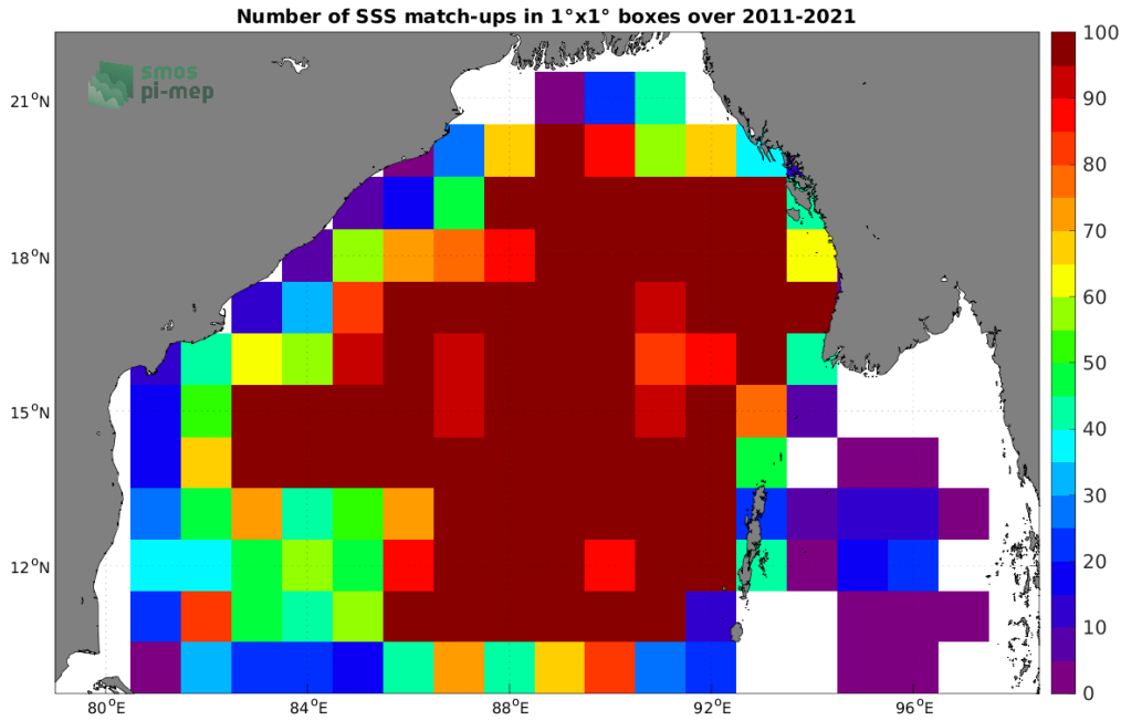
Figure 4: Number of SSS match-ups between Argo SSS and the SMOS SSS L3 v2 - 9-Days (BEC) SSS product for the Bay of Bengal Pi-MEP region over 1^{\circ} \times 1^{\circ} boxes and for the full satellite product period.
