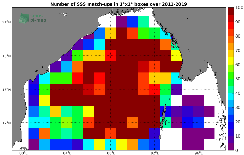
Figure 4: Number of SSS match-ups between Argo SSS and the SMOS SSS L3 v2 - 9-Days (BEC) SSS product for the Bay of Bengal Pi-MEP region over 1°x1° boxes and for the full satellite product period.
