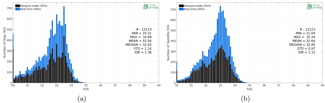
Figure 2: Histograms of SSS from Argo (a) and SMOS L3 v2 - 9-Days (BEC) (b) considering all match-up pairs per bins of 0.1 over the Bay of Bengal Pi-MEP region and for the full satellite product period.
