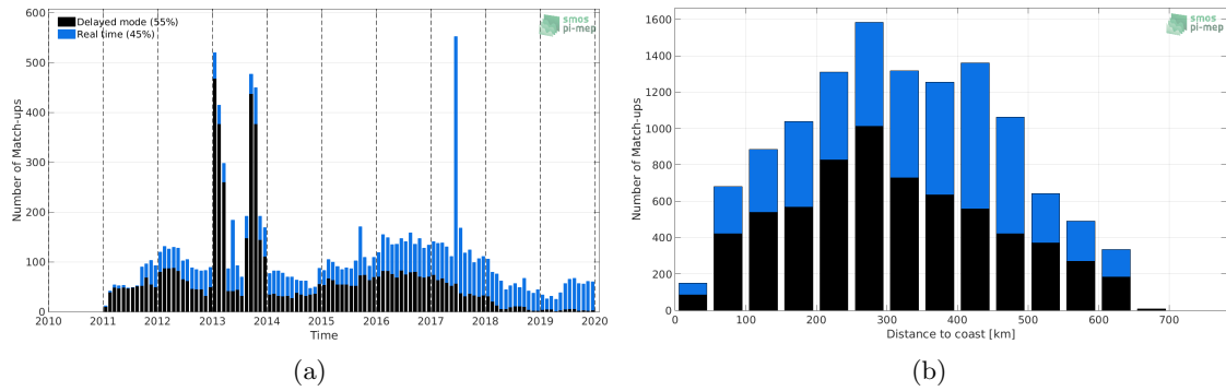
Figure 1: Number of match-ups between Argo and SMOS L3 v2 - 9-Days (BEC) SSS as a function of time (a) and as function of the distance to coast (b) over the Bay of Bengal Pi-MEP region and for the full satellite product period.
