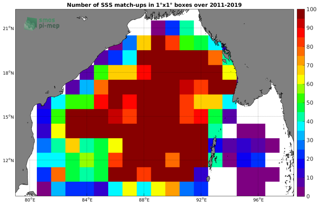
Figure 4: Number of SSS match-ups between Argo SSS and the SMOS L3 v2 - 9-Days (BEC) SSS product for the Bay of Bengal Pi-MEP region over 1°x1° boxes and for the full satellite product period.
