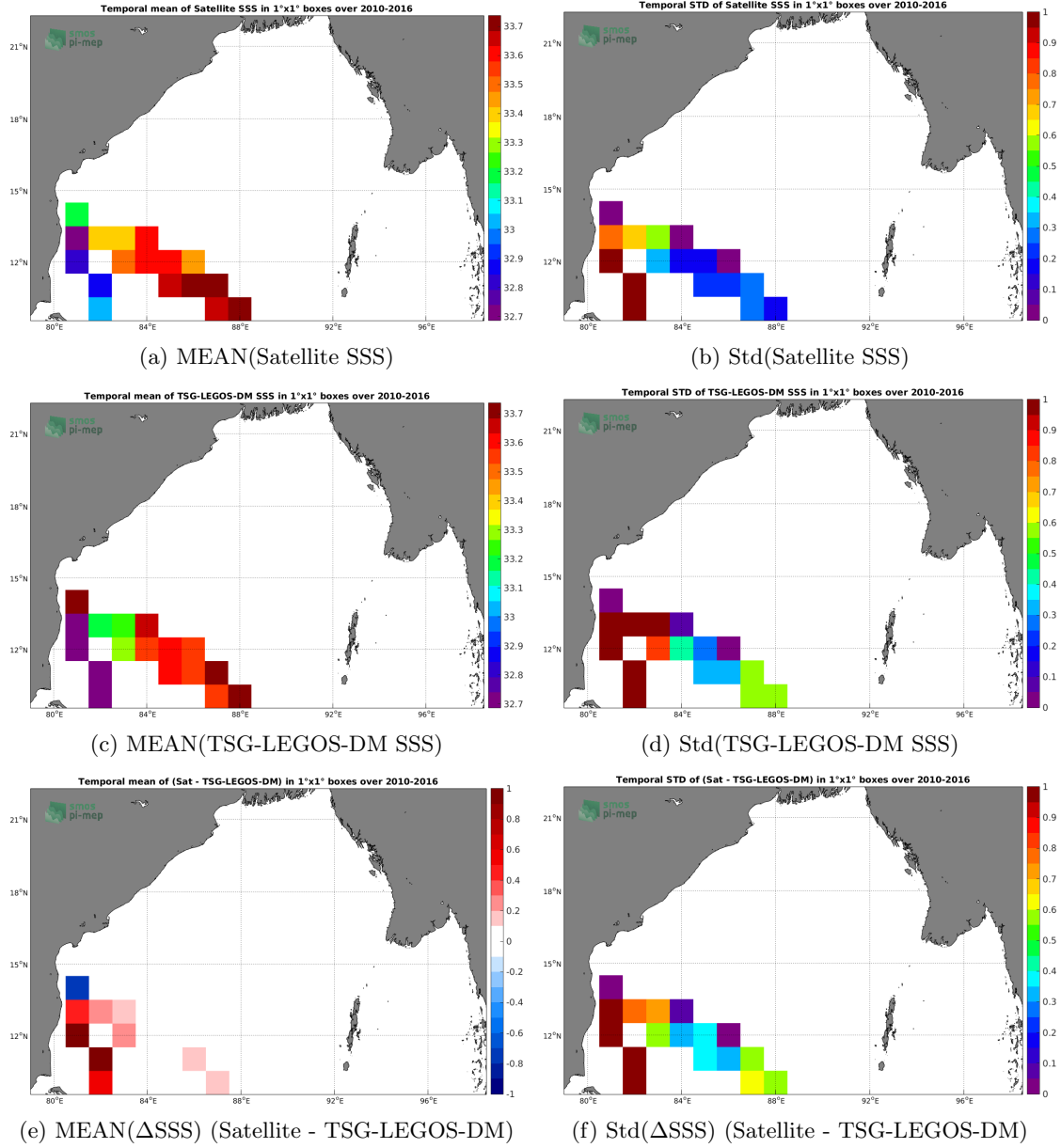
Figure 6: Temporal mean (left) and Std (right) of SSS from SMOS-L3-BEC-OA-V1-9DAYS-0.25DEG (top), TSG-LEGOS-DM (middle), and of \Delta SSS (Satellite - TSG-LEGOS-DM). Only match-up pairs are used to generate these maps.
