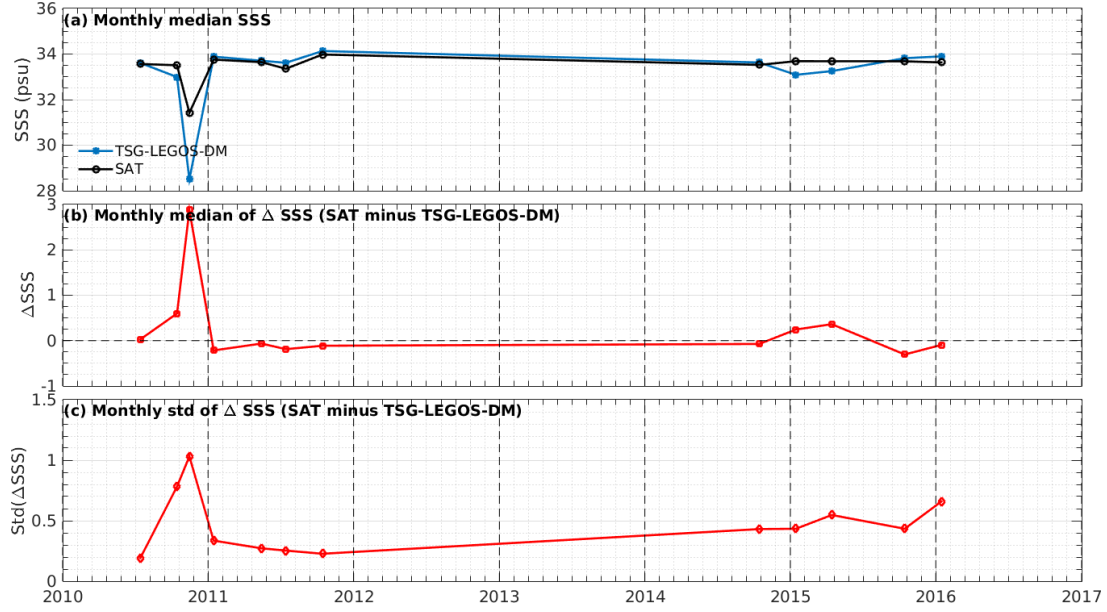
Figure 7: Time series of the monthly median SSS (top), median of \Delta SSS (Satellite - TSG-LEGOS-DM) and Std of \Delta SSS (Satellite - TSG-LEGOS-DM) over the Bay of Bengal Pi-MEP region considering all match-ups collected by the Pi-MEP.
