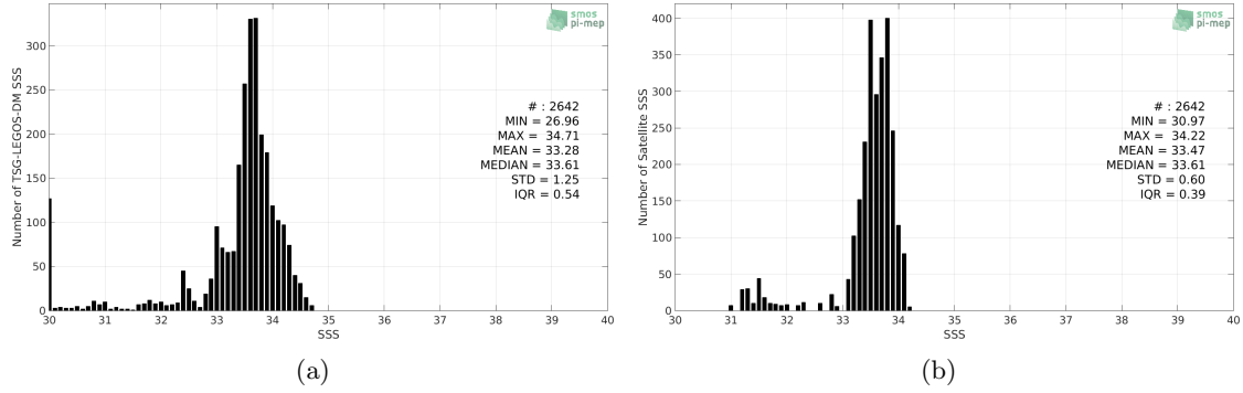
Figure 2: Histograms of SSS from TSG-LEGOS-DM (a) and SMOS-L3-BEC-OA-V1-9DAYS-0.25DEG (b) considering all match-up pairs per bins of 0.1 over the Bay of Bengal Pi-MEP region and for the full satellite product period.
