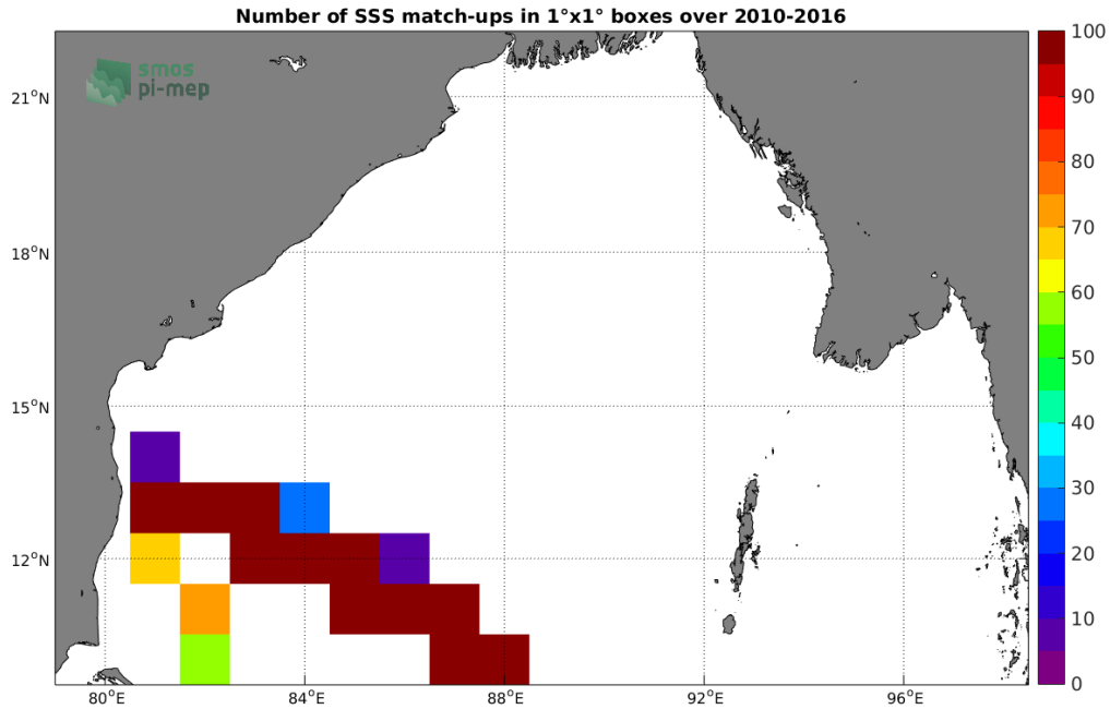
Figure 4: Number of SSS match-ups between TSG-LEGOS-DM SSS and the SMOS-L3-BEC-OA-V1-9DAYS-0.25DEG SSS product for the Bay of Bengal Pi-MEP region over 1°x1° boxes and for the full satellite product period.
