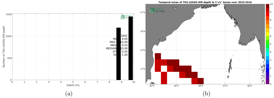
Figure 3: Histograms of the depth of the upper level SSS measurements from TSG-LEGOS-DM in the Match-up DataBase for the Bay of Bengal Pi-MEP region (a) and temporal mean spatial distribution of pressure of the in situ SSS data over 1°x1° boxes and for the full satellite product period (b).
