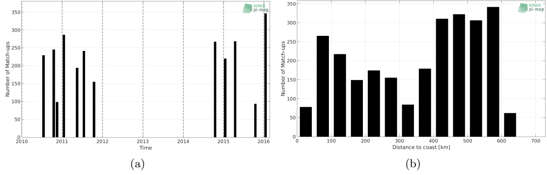
Figure 1: Number of match-ups between TSG-LEGOS-DM and SMOS-L3-BEC-OA-V1-9DAYS-0.25DEG SSS as a function of time (a) and as function of the distance to coast (b) over the Bay of Bengal Pi-MEP region and for the full satellite product period.
