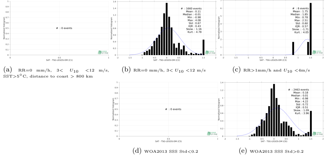
Figure 13: Normalized histogram of \Delta\text{SSS} (SMOS-L3-BEC-OA-V1-9DAYS-0.25DEG - TSG-LEGOS-DM) for 5 different subdatasets corresponding to: RR=0 mm/h, 3 < U_{10} < 12 m/s, SST > 5^\circ\text{C} , distance to coast > 800 km (a), RR=0 mm/h, 3 < U_{10} < 12 m/s (b), RR > 1 mm/h and U_{10} < 4 m/s (c), WOA2013 SSS Std < 0.2 (d), WOA2013 SSS Std > 0.2 (e).
