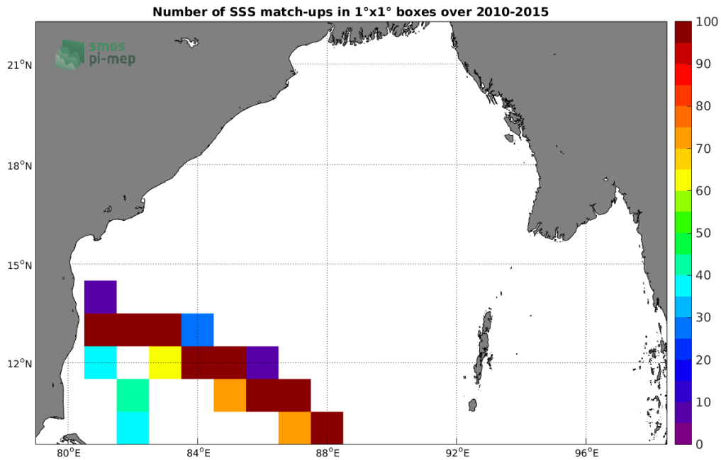
Figure 4: Number of SSS match-ups between TSG-LEGOS-DM SSS and the SMOS-L3-BEC-OA-V1-9DAYS-0.25DEG SSS product for the Bay of Bengal Pi-MEP region over 1^\circ \times 1^\circ boxes and for the full satellite product period.
