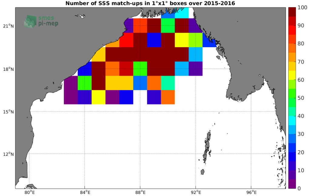
Figure 3: Number of SSS match-ups between Surface drifters SSS and the SMOS-L3-BEC-OA-V1-9DAYS-0.25DEG SSS product for the Bay of Bengal Pi-MEP region over 1^\circ \times 1^\circ boxes and for the full satellite product period.
