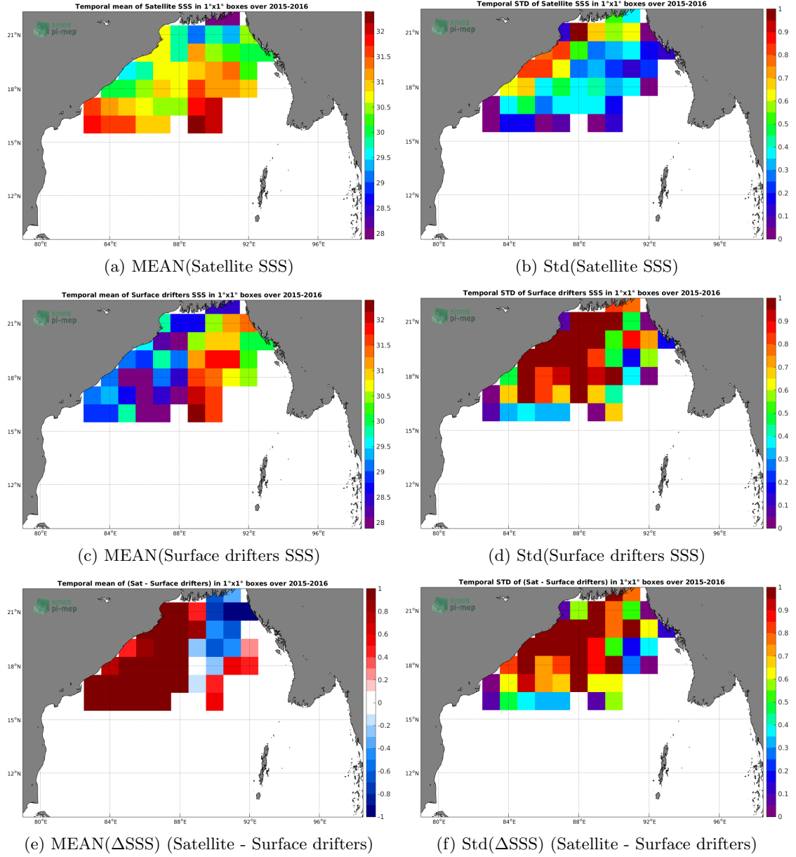
Figure 5: Temporal mean (left) and Std (right) of SSS from SMOS-L3-BEC-OA-V1-9DAYS-0.25DEG (top), Surface drifters (middle), and of \Delta SSS (Satellite - Surface drifters). Only match-up pairs are used to generate these maps.
