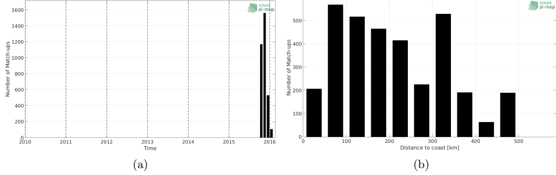
Figure 1: Number of match-ups between Surface drifters and SMOS-L3-BEC-OA-V1-9DAYS-0.25DEG SSS as a function of time (a) and as function of the distance to coast (b) over the Bay of Bengal Pi-MEP region and for the full satellite product period.
