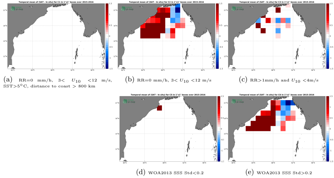
Figure 11: Temporal mean gridded over spatial boxes of size 1^\circ \times 1^\circ of \Delta SSS (SMOS-L3-BEC-OA-V1-9DAYS-0.25DEG - Surface drifters) for 5 different subdatasets corresponding to: RR=0 mm/h, 3 < U_{10} < 12 m/s, SST > 5^\circ C , distance to coast > 800 km (a), RR=0 mm/h, 3 < U_{10} < 12 m/s (b), RR > 1 mm/h and U_{10} < 4 m/s (c), WOA2013 SSS Std < 0.2 (d), WOA2013 SSS Std > 0.2 (e).
