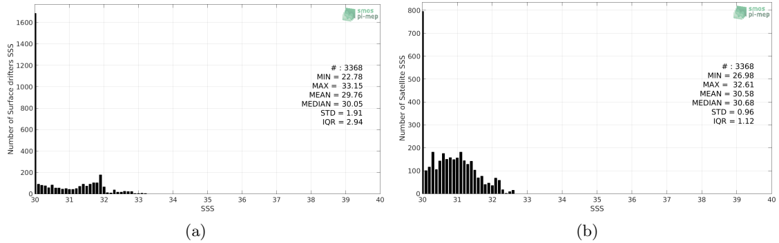
Figure 2: Histograms of SSS from Surface drifters (a) and SMOS-L3-BEC-OA-V1-9DAYS-0.25DEG (b) considering all match-up pairs per bins of 0.1 over the Bay of Bengal Pi-MEP region and for the full satellite product period.
