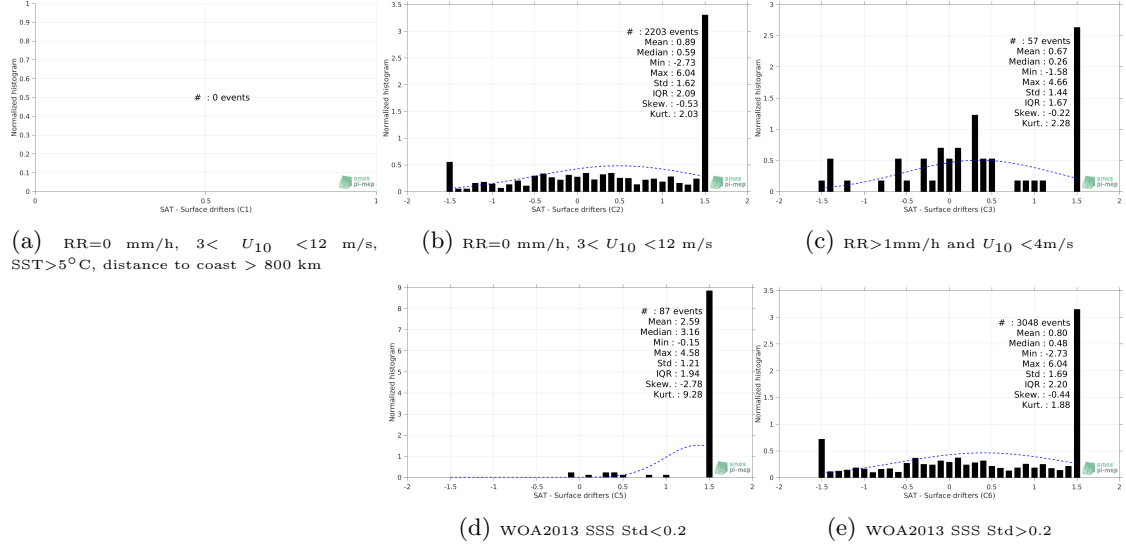
Figure 12: Normalized histogram of \Delta SSS (SMOS-L3-BEC-OA-V1-9DAYS-0.25DEG - Surface drifters) for 5 different subdatasets corresponding to: RR=0 mm/h, 3 < U_{10} < 12 m/s, SST>5°C, distance to coast > 800 km (a), RR=0 mm/h, 3 < U_{10} < 12 m/s (b), RR>1mm/h and U_{10} < 4 m/s (c), WOA2013 SSS Std<0.2 (d), WOA2013 SSS Std>0.2 (e).
