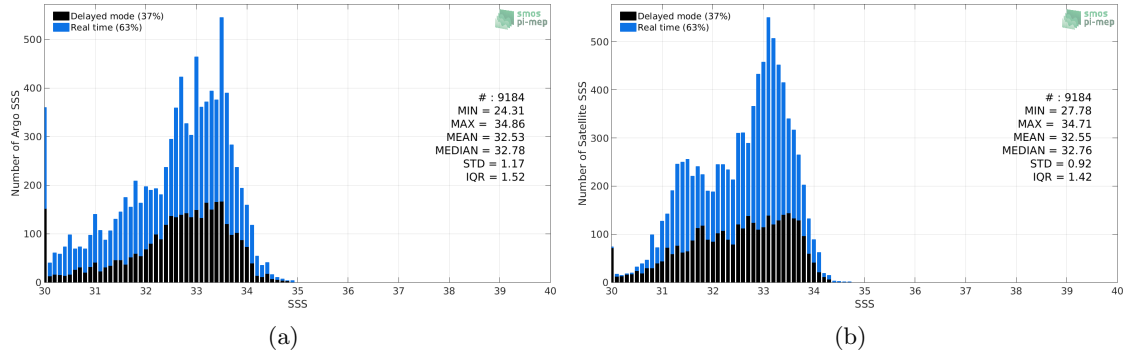
Figure 2: Histograms of SSS from Argo (a) and SMOS-L3-BEC-OA-V1-9DAYS-0.25DEG (b) considering all match-up pairs per bins of 0.1 over the Bay of Bengal Pi-MEP region and for the full satellite product period.
