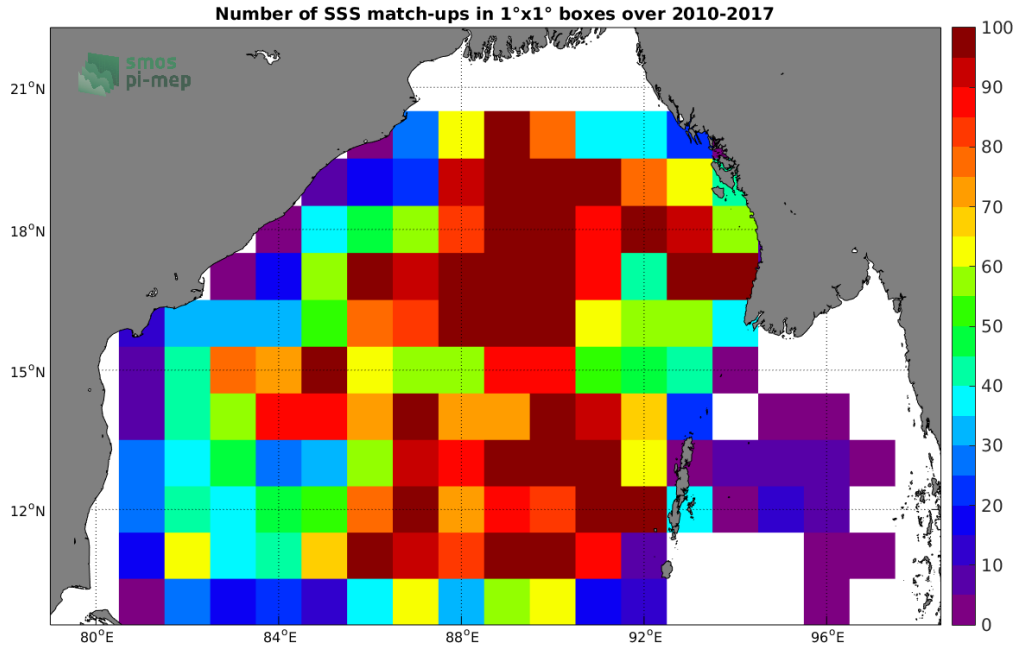
Figure 4: Number of SSS match-ups between Argo SSS and the SMOS-L3-BEC-OA-V1-9DAYS-0.25DEG SSS product for the Bay of Bengal Pi-MEP region over 1^\circ \times 1^\circ boxes and for the full satellite product period.
