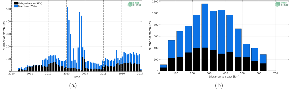
Figure 1: Number of match-ups between Argo and SMOS-L3-BEC-OA-V1-9DAYS-0.25DEG SSS as a function of time (a) and as function of the distance to coast (b) over the Bay of Bengal Pi-MEP region and for the full satellite product period.
