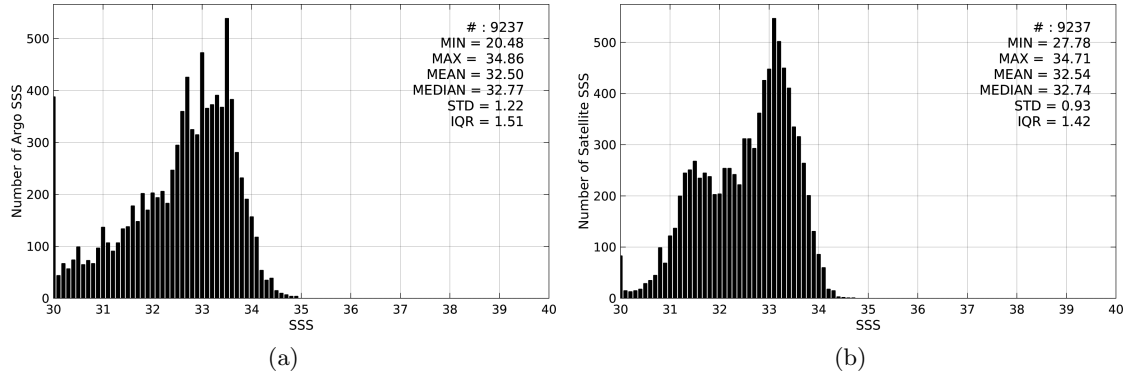
Figure 2: Histograms of SSS from Argo (a) and SMOS-L3-BEC-OA-V1-9DAYS-0.25DEG (b) considering all match-up pairs per bins of 0.1 over the Bay of Bengal Pi-MEP region and for the full satellite product period.
