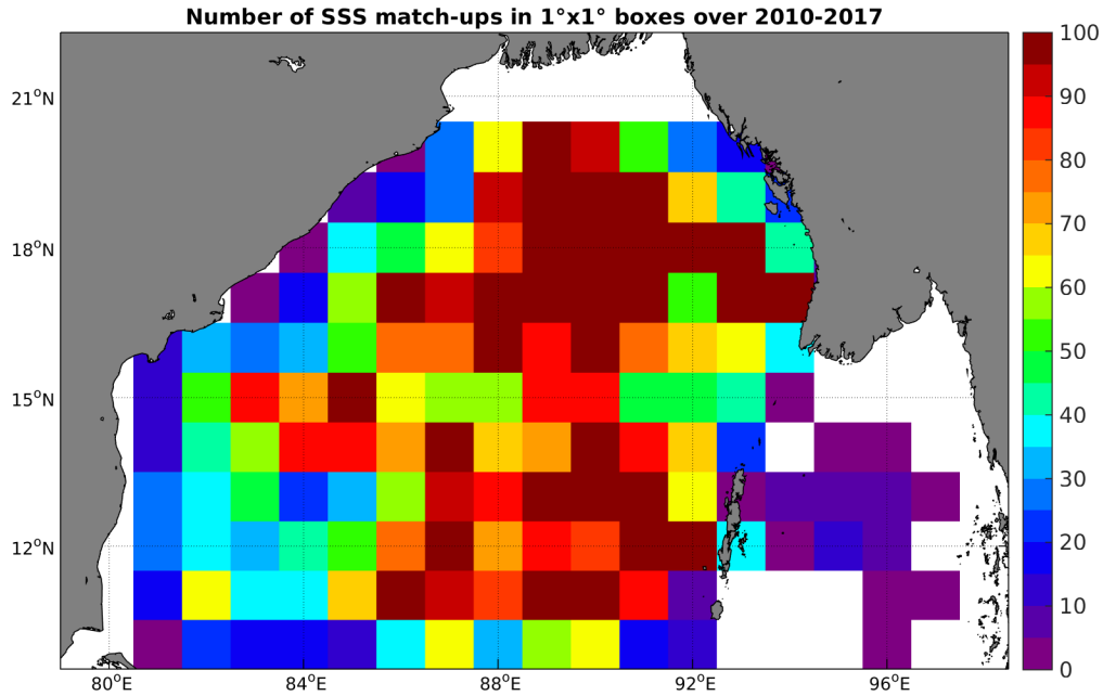
Figure 4: Number of SSS match-ups between Argo SSS and the SMOS-L3-BEC-OA-V1-9DAYS-0.25DEG SSS product for the Bay of Bengal Pi-MEP region over 1°x1° boxes and for the full satellite product period.
