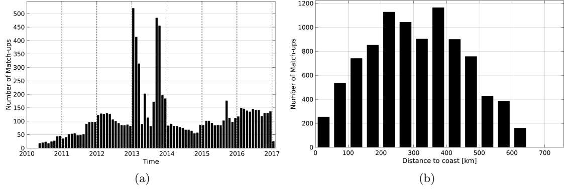
Figure 1: Number of match-ups between Argo and SMOS-L3-BEC-OA-V1-9DAYS-0.25DEG SSS as a function of time (a) and as function of the distance to coast (b) over the Bay of Bengal Pi-MEP region and for the full satellite product period.
