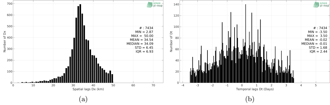
Figure 5: Histograms of the spatial (a) and temporal (b) lags between the location/time of the Argo measurement and the date of the corresponding SMOS SSS L2-AVERAGED v700 (ESA) SSS pixel.
