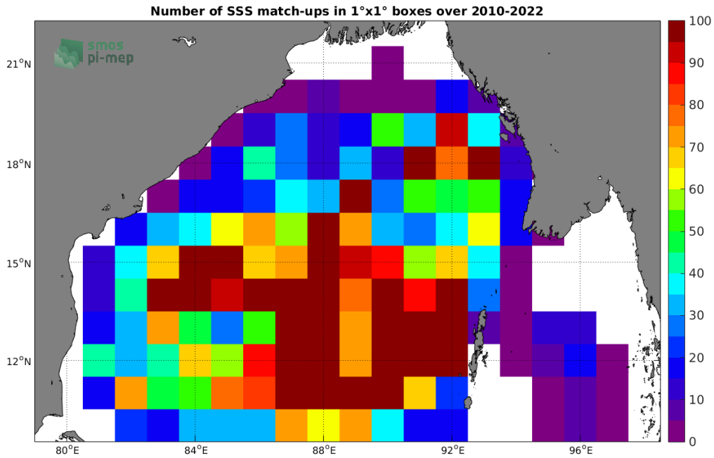
Figure 4: Number of SSS match-ups between Argo SSS and the SMOS SSS L2-AVERAGED v700 (ESA) SSS product for the Bay of Bengal Pi-MEP region over 1°×1° boxes and for the full satellite product period.
