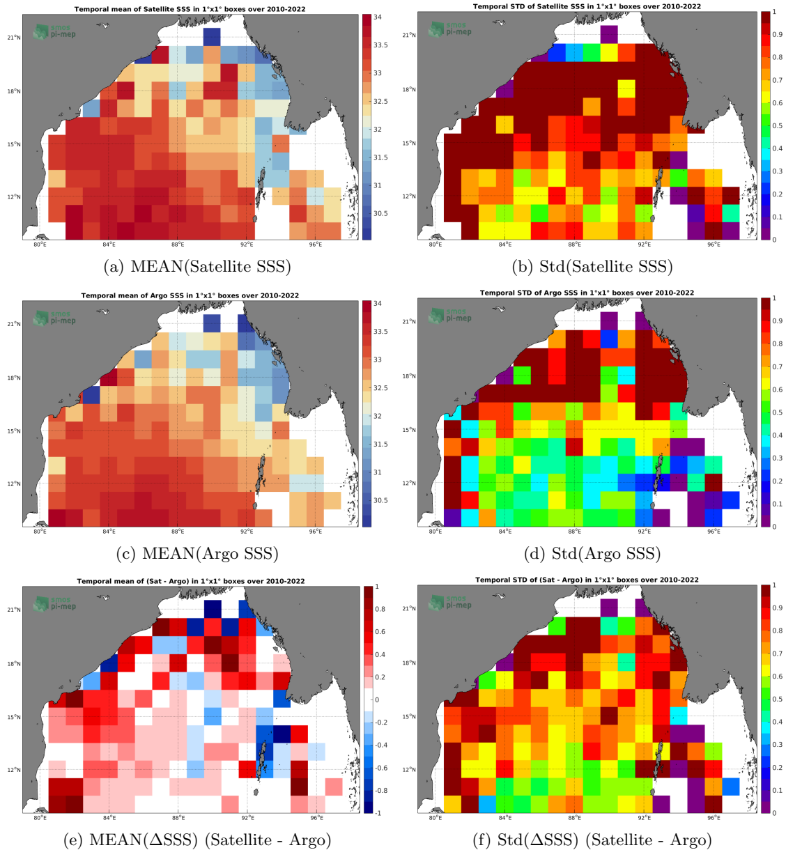
Figure 6: Temporal mean (left) and Std (right) of SSS from SMOS SSS L2-AVERAGED v700 (ESA) (top), Argo (middle), and of \Delta SSS (Satellite - Argo). Only match-up pairs are used to generate these maps.
