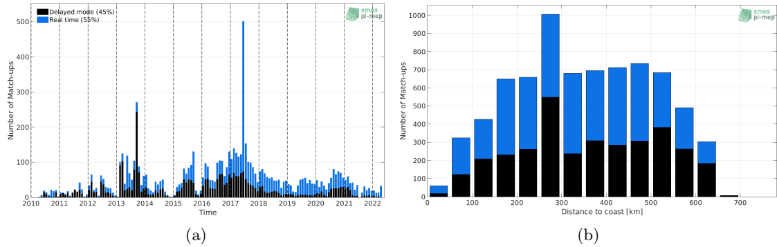
Figure 1: Number of match-ups between Argo and SMOS SSS L2-AVERAGED v700 (ESA) SSS as a function of time (a) and as function of the distance to coast (b) over the Bay of Bengal Pi-MEP region and for the full satellite product period.
