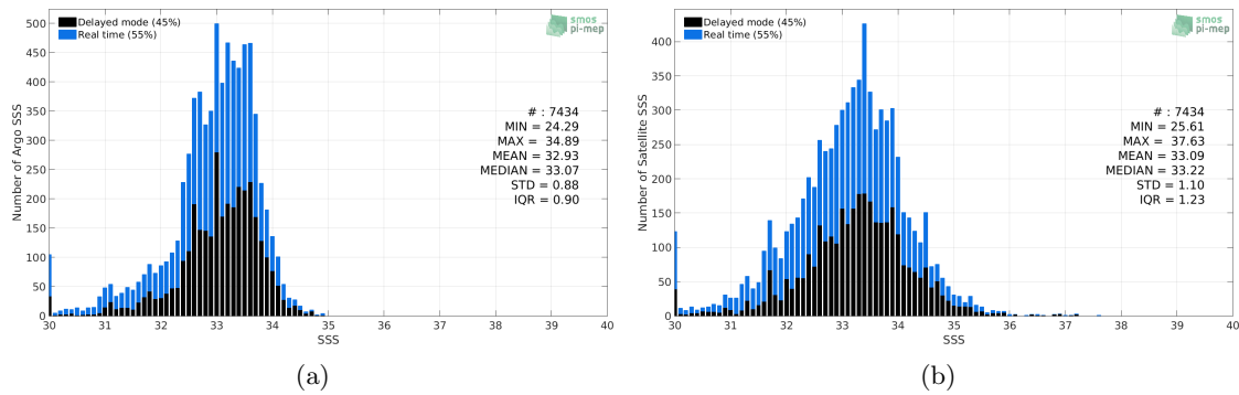
Figure 2: Histograms of SSS from Argo (a) and SMOS SSS L2-AVERAGED v700 (ESA) (b) considering all match-up pairs per bins of 0.1 over the Bay of Bengal Pi-MEP region and for the full satellite product period.
