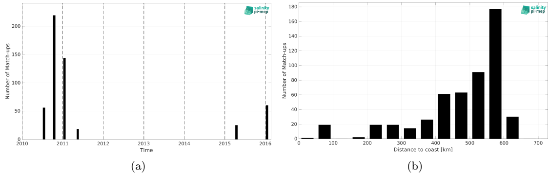
Figure 2: Number of match-ups between TSG (LEGOS-DM) and SMOS SSS L2 v700 (ESA) SSS as a function of time (a) and as function of the distance to coast (b) over the Bay of Bengal Pi-MEP region and for the full satellite product period.
