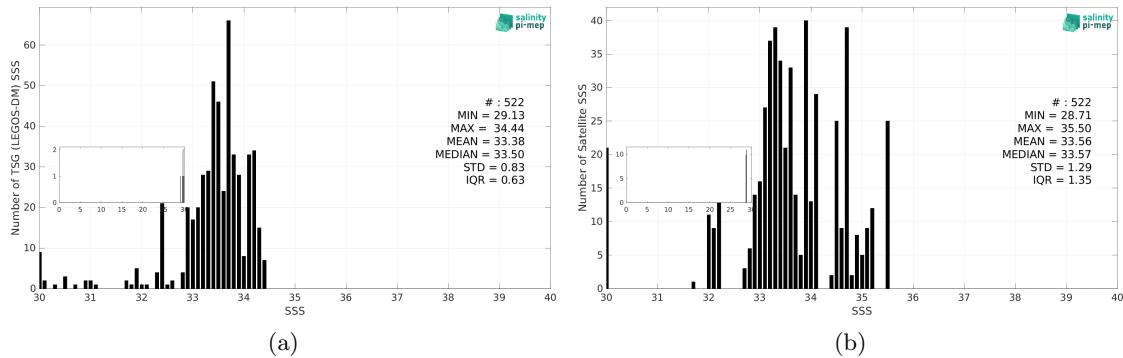
Figure 3: Histograms of SSS from TSG (LEGOS-DM) (a) and SMOS SSS L2 v700 (ESA) (b) considering all match-up pairs per bins of 0.1 over the Bay of Bengal Pi-MEP region and for the full satellite product period.
