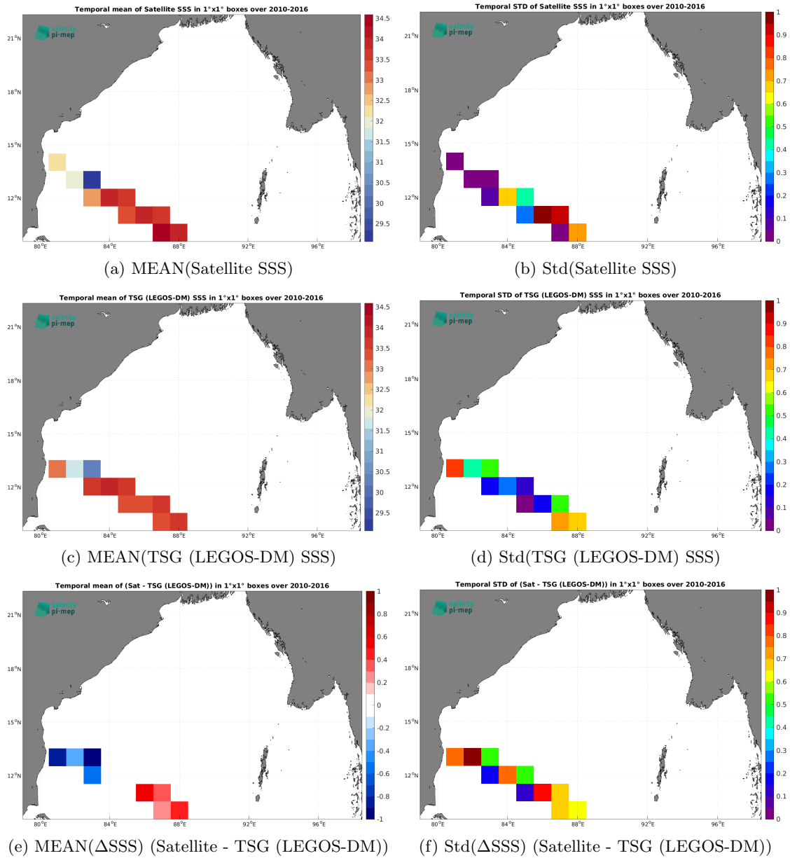
Figure 7: Temporal mean (left) and Std (right) of SSS from SMOS SSS L2 v700 (ESA) (top), TSG (LEGOS-DM) (middle), and of \Delta SSS (Satellite - TSG (LEGOS-DM)). Only match-up pairs are used to generate these maps.
