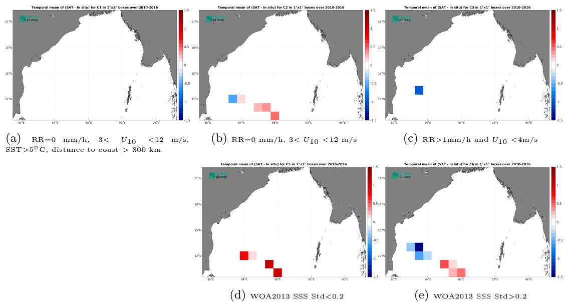
Figure 14: Temporal mean gridded over spatial boxes of size 1^\circ \times 1^\circ of \Delta SSS (SMOS SSS L2 v700 (ESA) - TSG (LEGOS-DM)) for 5 different subdatasets corresponding to:RR=0 mm/h, 3 < U_{10} < 12 m/s, SST>5°C, distance to coast > 800 km (a), RR=0 mm/h, 3 < U_{10} < 12 m/s (b), RR>1mm/h and U_{10} < 4 m/s (c), WOA2013 SSS Std<0.2 (d), WOA2013 SSS Std>0.2 (e).
