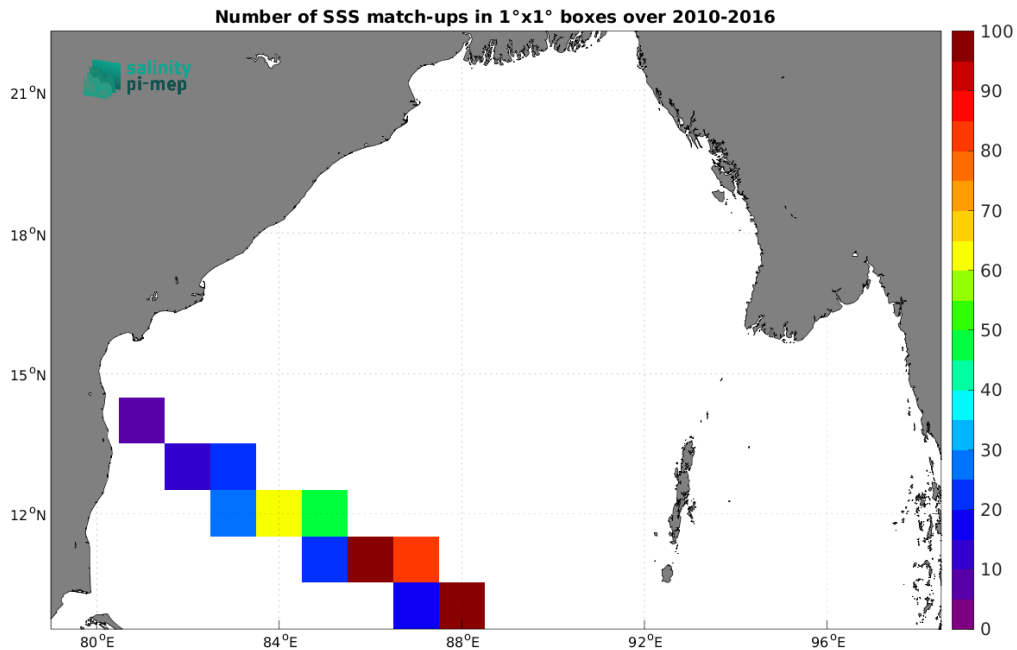
Figure 5: Number of SSS match-ups between TSG (LEGOS-DM) SSS and the SMOS SSS L2 v700 (ESA) SSS product for the Bay of Bengal Pi-MEP region over 1^\circ \times 1^\circ boxes and for the full satellite product period.
