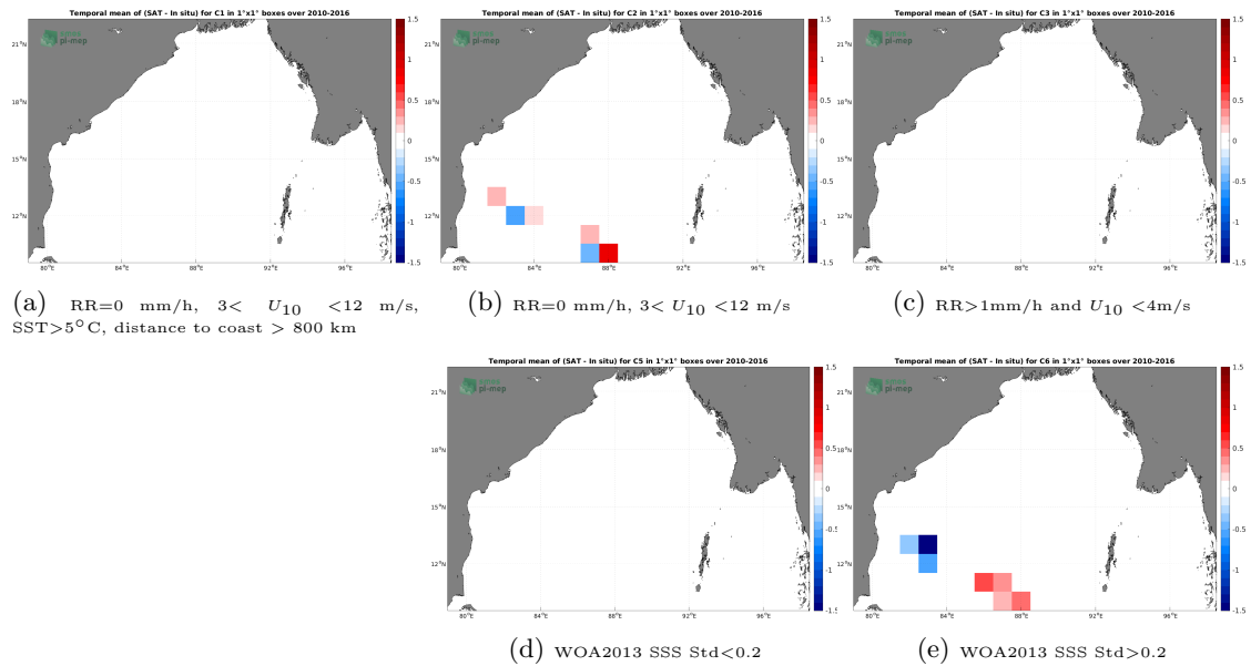
Figure 12: Temporal mean gridded over spatial boxes of size 1^\circ \times 1^\circ of \Delta SSS (SMOS SSS L2 v700 (ESA) - TSG (LEGOS-DM)) for 5 different subdatasets corresponding to:RR=0 mm/h, 3 < U_{10} < 12 m/s, SST >5^\circ\text{C} , distance to coast > 800 km (a), RR=0 mm/h, 3 < U_{10} < 12 m/s (b), RR >1 mm/h and U_{10} < 4 m/s (c), WOA2013 SSS Std <0.2 (d), WOA2013 SSS Std >0.2 (e).
