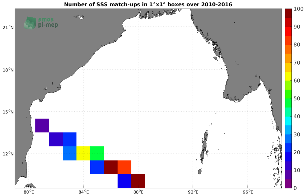
Figure 4: Number of SSS match-ups between TSG (LEGOS-DM) SSS and the SMOS SSS L2 v700 (ESA) SSS product for the Bay of Bengal Pi-MEP region over 1^\circ \times 1^\circ boxes and for the full satellite product period.
