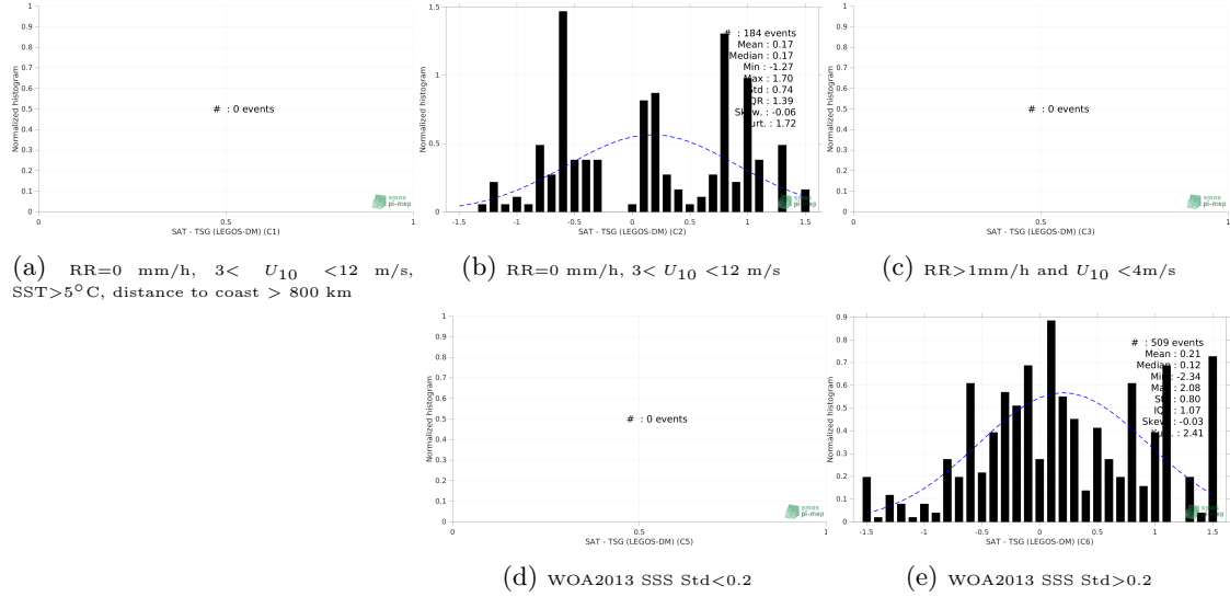
Figure 13: Normalized histogram of \Delta SSS (SMOS SSS L2 v700 (ESA) - TSG (LEGOS-DM)) for 5 different subdatasets corresponding to: RR=0 mm/h, 3 < U_{10} < 12 m/s, SST > 5°C, distance to coast > 800 km (a), RR=0 mm/h, 3 < U_{10} < 12 m/s (b), RR > 1mm/h and U_{10} < 4 m/s (c), WOA2013 SSS Std < 0.2 (d), WOA2013 SSS Std > 0.2 (e).
