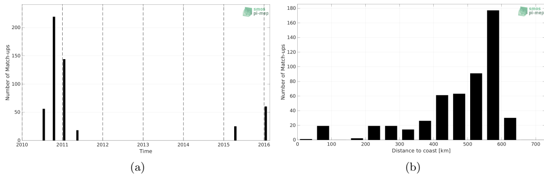
Figure 1: Number of match-ups between TSG (LEGOS-DM) and SMOS SSS L2 v700 (ESA) SSS as a function of time (a) and as function of the distance to coast (b) over the Bay of Bengal Pi-MEP region and for the full satellite product period.
