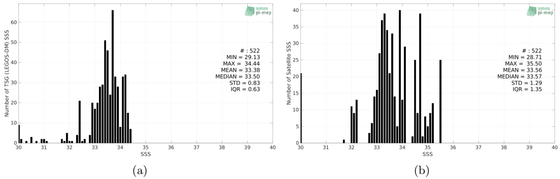
Figure 2: Histograms of SSS from TSG (LEGOS-DM) (a) and SMOS SSS L2 v700 (ESA) (b) considering all match-up pairs per bins of 0.1 over the Bay of Bengal Pi-MEP region and for the full satellite product period.
