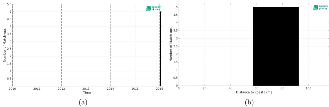
Figure 2: Number of match-ups between Surface drifters and SMOS SSS L2 v700 (ESA) SSS as a function of time (a) and as function of the distance to coast (b) over the Bay of Bengal Pi-MEP region and for the full satellite product period.
