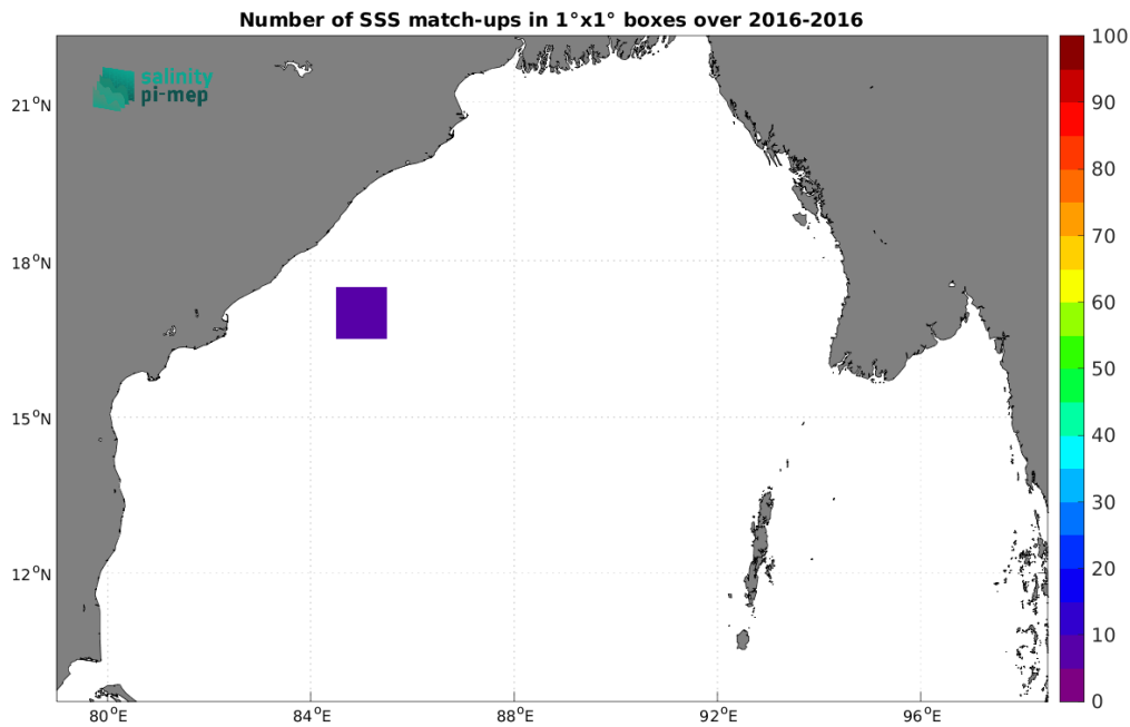
Figure 4: Number of SSS match-ups between Surface drifters SSS and the SMOS SSS L2 v700 (ESA) SSS product for the Bay of Bengal Pi-MEP region over 1°x1° boxes and for the full satellite product period.
