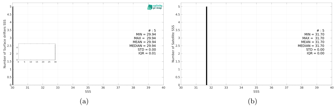
Figure 3: Histograms of SSS from Surface drifters (a) and SMOS SSS L2 v700 (ESA) (b) considering all match-up pairs per bins of 0.1 over the Bay of Bengal Pi-MEP region and for the full satellite product period.
