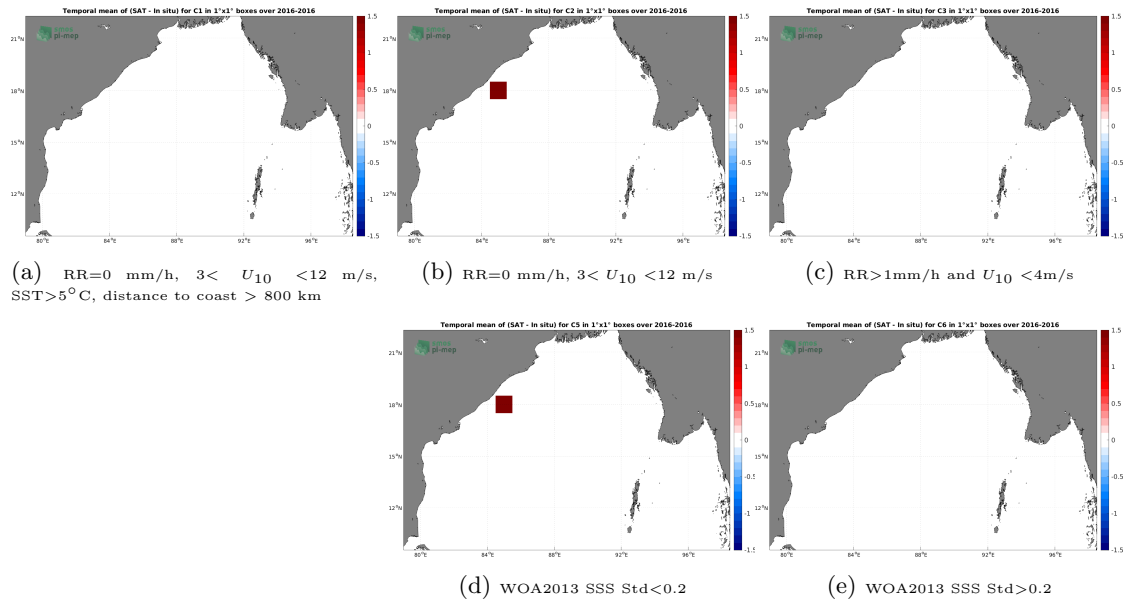
Figure 11: Temporal mean gridded over spatial boxes of size 1^{\circ}\times 1^{\circ} of \Delta\text{SSS} (SMOS SSS L2 v700 (ESA) - Surface drifters) for 5 different subdatasets corresponding to:RR=0 mm/h, 3 < U_{10} < 12 m/s, SST > 5^{\circ}\text{C} , distance to coast > 800 km (a), RR=0 mm/h, 3 < U_{10} < 12 m/s (b), RR > 1 mm/h and U_{10} < 4 m/s (c), WOA2013 SSS Std < 0.2 (d), WOA2013 SSS Std > 0.2 (e).
