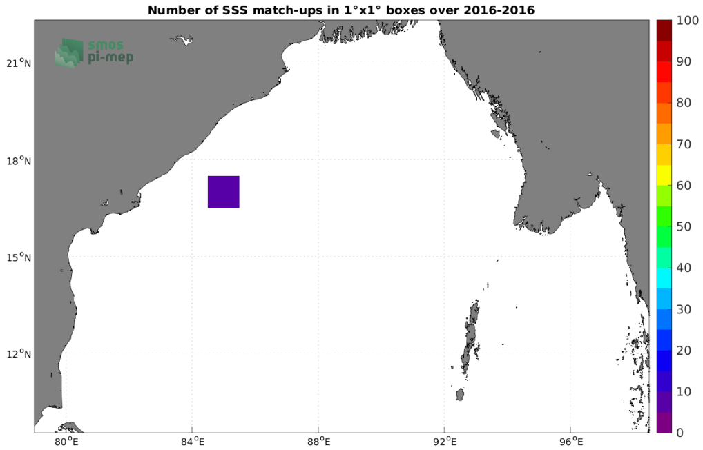
Figure 3: Number of SSS match-ups between Surface drifters SSS and the SMOS SSS L2 v700 (ESA) SSS product for the Bay of Bengal Pi-MEP region over 1°x1° boxes and for the full satellite product period.
