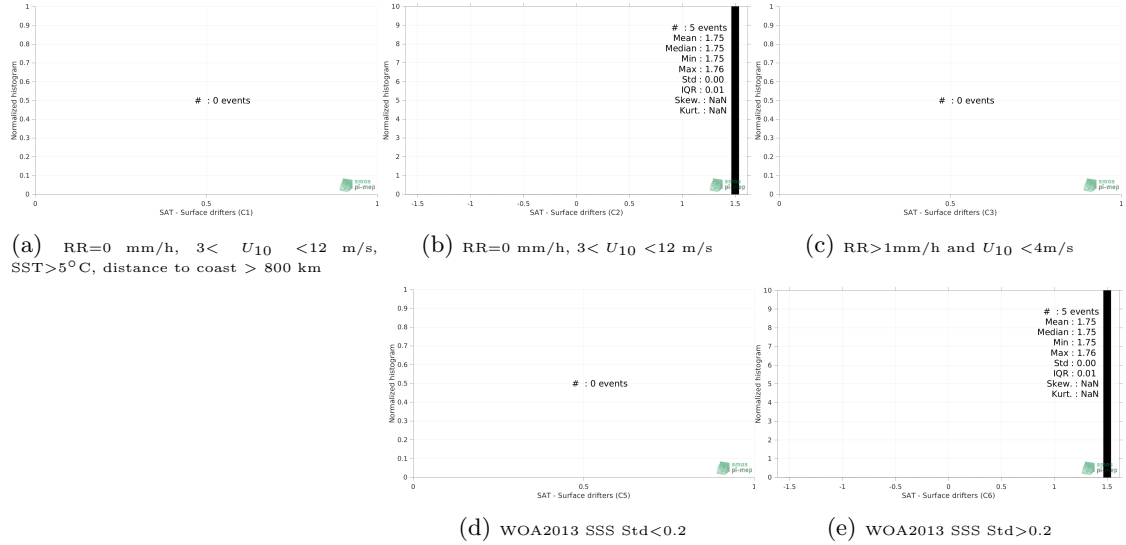
Figure 12: Normalized histogram of \Delta SSS (SMOS SSS L2 v700 (ESA) - Surface drifters) for 5 different subdatasets corresponding to: RR=0 mm/h, 3 < U_{10} < 12 m/s, SST > 5°C, distance to coast > 800 km (a), RR=0 mm/h, 3 < U_{10} < 12 m/s (b), RR > 1mm/h and U_{10} < 4 m/s (c), WOA2013 SSS Std < 0.2 (d), WOA2013 SSS Std > 0.2 (e).
