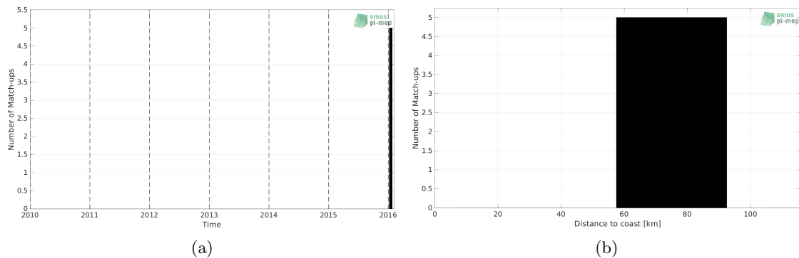
Figure 1: Number of match-ups between Surface drifters and SMOS SSS L2 v700 (ESA) SSS as a function of time (a) and as function of the distance to coast (b) over the Bay of Bengal Pi-MEP region and for the full satellite product period.
