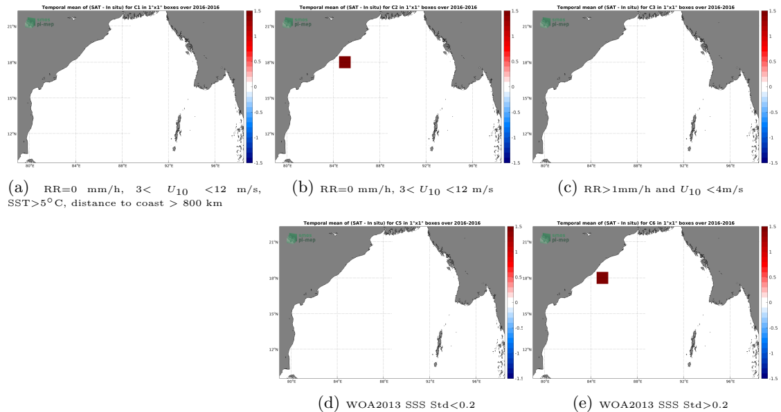
Figure 11: Temporal mean gridded over spatial boxes of size 1^{\circ}\times 1^{\circ} of \Delta\text{SSS} (SMOS SSS L2 v700 (ESA) - Surface drifters) for 5 different subdatasets corresponding to:RR=0 mm/h, 3 < U_{10} < 12 m/s, SST >5^{\circ}\text{C} , distance to coast > 800 km (a), RR=0 mm/h, 3 < U_{10} < 12 m/s (b), RR >1 mm/h and U_{10} < 4 m/s (c), WOA2013 SSS Std <0.2 (d), WOA2013 SSS Std >0.2 (e).
