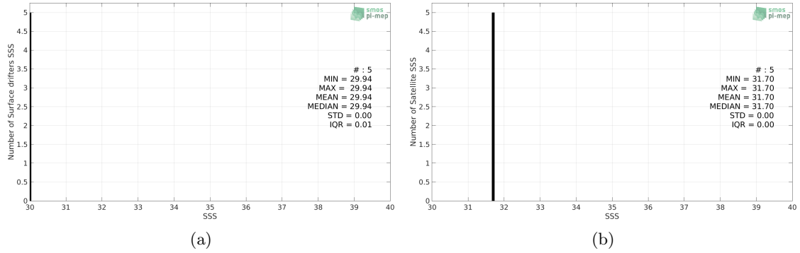
Figure 2: Histograms of SSS from Surface drifters (a) and SMOS SSS L2 v700 (ESA) (b) considering all match-up pairs per bins of 0.1 over the Bay of Bengal Pi-MEP region and for the full satellite product period.
