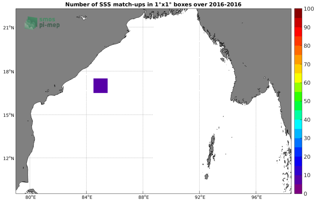
Figure 3: Number of SSS match-ups between Surface drifters SSS and the SMOS SSS L2 v700 (ESA) SSS product for the Bay of Bengal Pi-MEP region over 1^{\circ} \times 1^{\circ} boxes and for the full satellite product period.
