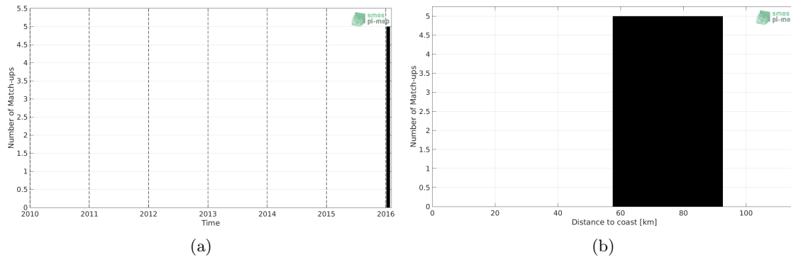
Figure 1: Number of match-ups between Surface drifters and SMOS SSS L2 v700 (ESA) SSS as a function of time (a) and as function of the distance to coast (b) over the Bay of Bengal Pi-MEP region and for the full satellite product period.
