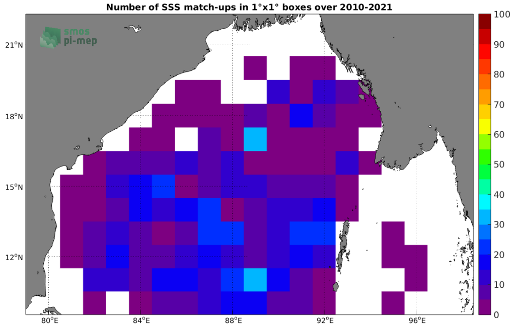
Figure 4: Number of SSS match-ups between Argo SSS and the SMOS SSS L2 v700 (ESA) SSS product for the Bay of Bengal Pi-MEP region over 1°x1° boxes and for the full satellite product period.
