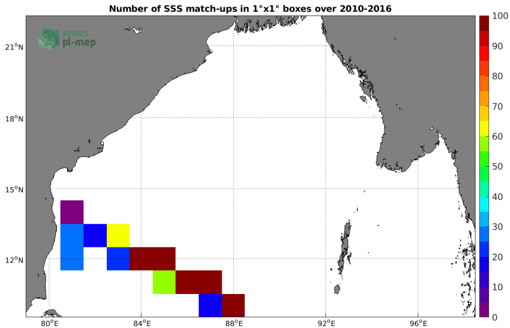
Figure 4: Number of SSS match-ups between TSG (LEGOS-DM) SSS and the SMOS SSS L2 v662 (ESA) SSS product for the Bay of Bengal Pi-MEP region over 1^\circ \times 1^\circ boxes and for the full satellite product period.
