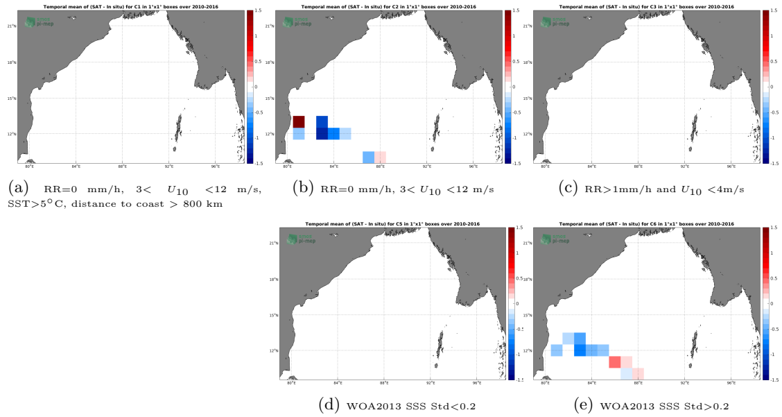
Figure 12: Temporal mean gridded over spatial boxes of size 1^\circ \times 1^\circ of \Delta SSS (SMOS SSS L2 v662 (ESA) - TSG (LEGOS-DM)) for 5 different subdatasets corresponding to: RR=0 mm/h, 3 < U_{10} < 12 m/s, SST>5°C, distance to coast > 800 km (a), RR=0 mm/h, 3 < U_{10} < 12 m/s (b), RR>1mm/h and U_{10} < 4 m/s (c), WOA2013 SSS Std<0.2 (d), WOA2013 SSS Std>0.2 (e).
