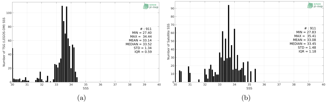
Figure 2: Histograms of SSS from TSG (LEGOS-DM) (a) and SMOS SSS L2 v662 (ESA) (b) considering all match-up pairs per bins of 0.1 over the Bay of Bengal Pi-MEP region and for the full satellite product period.
