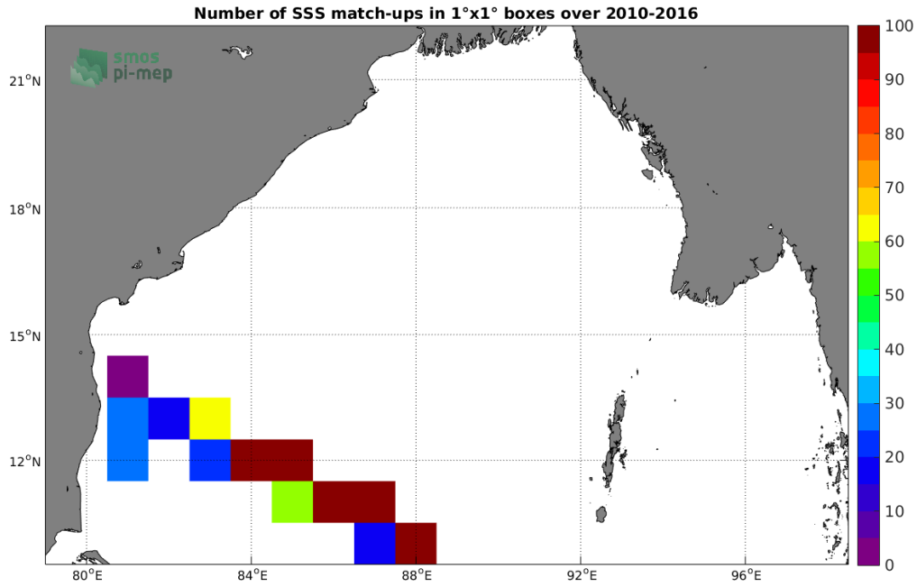
Figure 4: Number of SSS match-ups between TSG (LEGOS-DM) SSS and the SMOS SSS L2 v662 (ESA) SSS product for the Bay of Bengal Pi-MEP region over 1°x1° boxes and for the full satellite product period.
