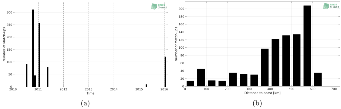
Figure 1: Number of match-ups between TSG (LEGOS-DM) and SMOS SSS L2 v662 (ESA) SSS as a function of time (a) and as function of the distance to coast (b) over the Bay of Bengal Pi-MEP region and for the full satellite product period.
