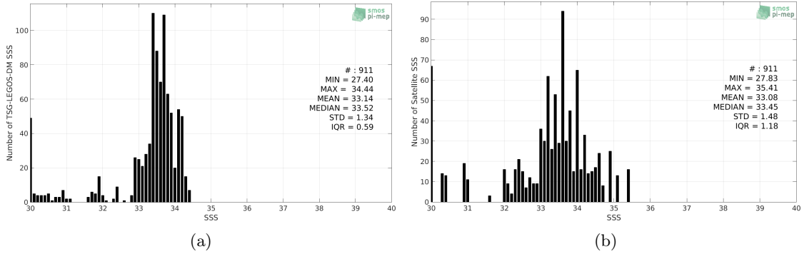
Figure 2: Histograms of SSS from TSG-LEGOS-DM (a) and SMOS L2 v662 (ESA) (b) considering all match-up pairs per bins of 0.1 over the Bay of Bengal Pi-MEP region and for the full satellite product period.
