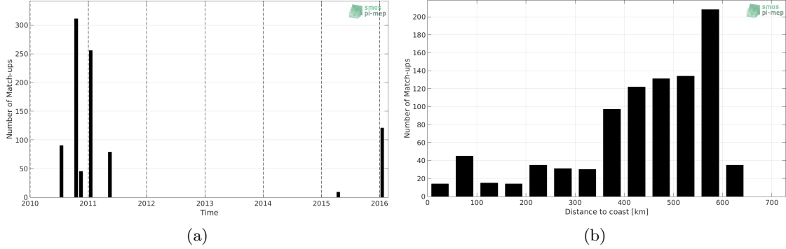
Figure 1: Number of match-ups between TSG-LEGOS-DM and SMOS L2 v662 (ESA) SSS as a function of time (a) and as function of the distance to coast (b) over the Bay of Bengal Pi-MEP region and for the full satellite product period.
