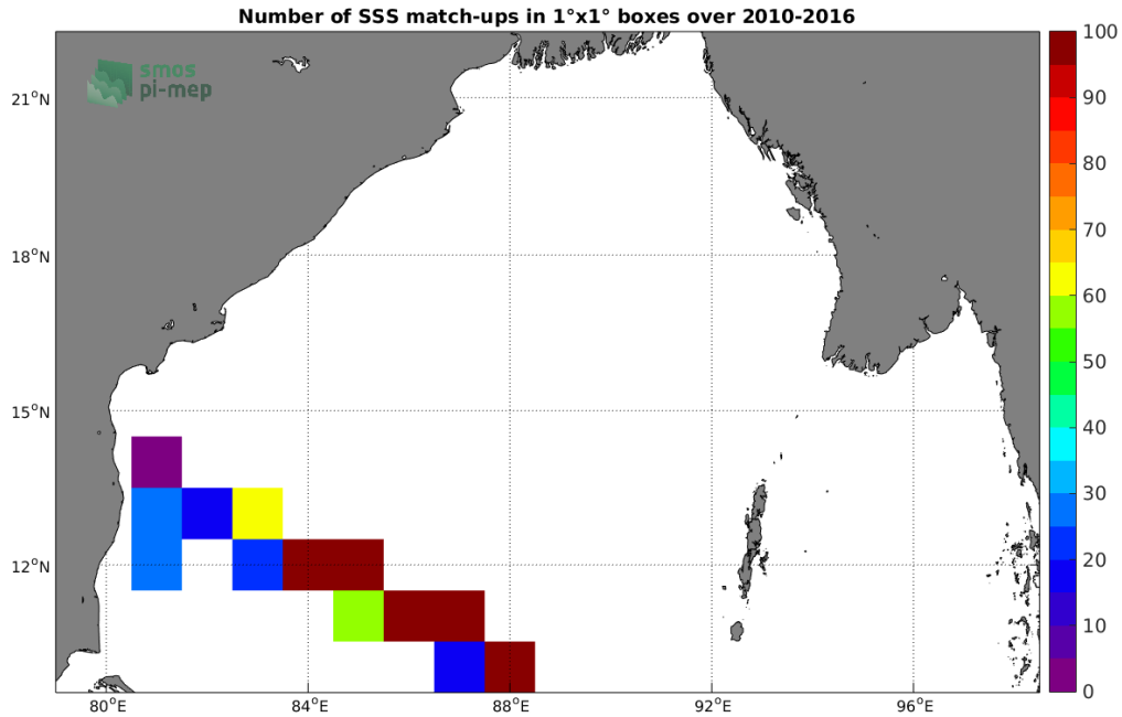
Figure 4: Number of SSS match-ups between TSG-LEGOS-DM SSS and the SMOS L2 v662 (ESA) SSS product for the Bay of Bengal Pi-MEP region over 1°x1° boxes and for the full satellite product period.
