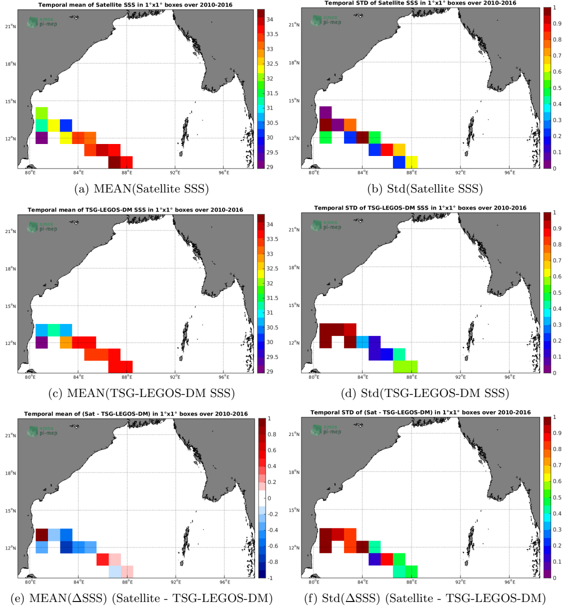
Figure 6: Temporal mean (left) and Std (right) of SSS from SMOS-L2-DPGS-v662 (top), TSG-LEGOS-DM (middle), and of \Delta SSS (Satellite - TSG-LEGOS-DM). Only match-up pairs are used to generate these maps.
