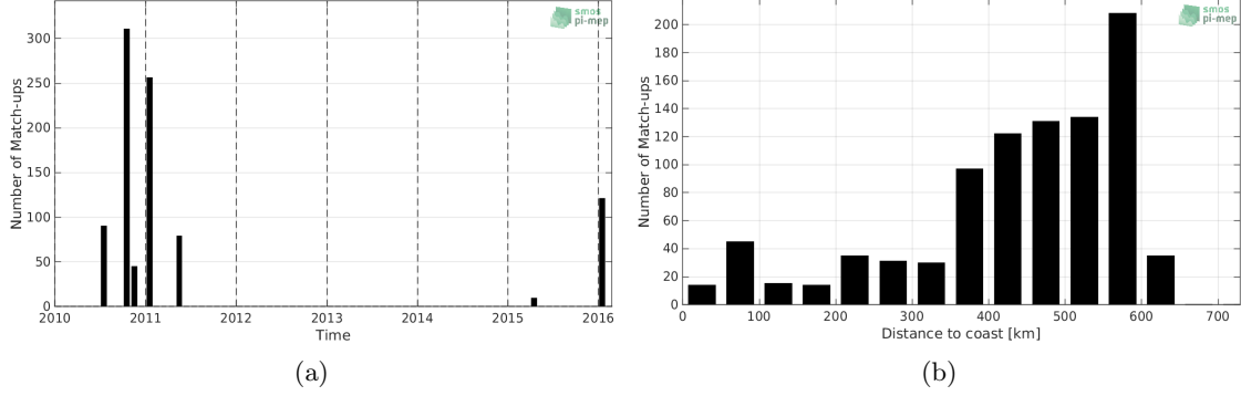
Figure 1: Number of match-ups between TSG-LEGOS-DM and SMOS-L2-DPGS-v662 SSS as a function of time (a) and as function of the distance to coast (b) over the Bay of Bengal Pi-MEP region and for the full satellite product period.
