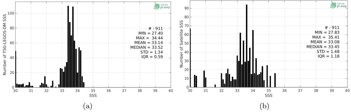
Figure 2: Histograms of SSS from TSG-LEGOS-DM (a) and SMOS-L2-DPGS-v662 (b) considering all match-up pairs per bins of 0.1 over the Bay of Bengal Pi-MEP region and for the full satellite product period.
