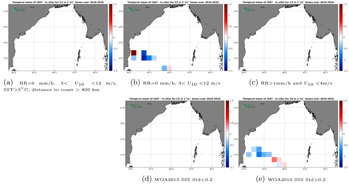
Figure 12: Temporal mean gridded over spatial boxes of size 1^\circ \times 1^\circ of \Delta SSS (SMOS-L2-DPGS-v662 - TSG-LEGOS-DM) for 5 different subdatasets corresponding to: RR=0 mm/h, 3 < U_{10} < 12 m/s, SST > 5^\circ\text{C} , distance to coast > 800 km (a), RR=0 mm/h, 3 < U_{10} < 12 m/s (b), RR > 1 mm/h and U_{10} < 4 m/s (c), WOA2013 SSS Std < 0.2 (d), WOA2013 SSS Std > 0.2 (e).
