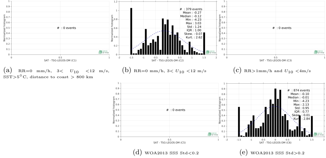
Figure 13: Normalized histogram of \Delta SSS (SMOS-L2-DPGS-v662 - TSG-LEGOS-DM) for 5 different subdatasets corresponding to: RR=0 mm/h, 3 < U_{10} < 12 m/s, SST>5°C, distance to coast > 800 km (a), RR=0 mm/h, 3 < U_{10} < 12 m/s (b), RR>1 mm/h and U_{10} < 4 m/s (c), WOA2013 SSS Std<0.2 (d), WOA2013 SSS Std>0.2 (e).
