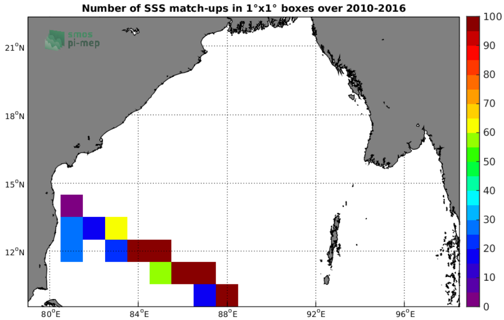
Figure 4: Number of SSS match-ups between TSG-LEGOS-DM SSS and the SMOS-L2-DPGS-v662 SSS product for the Bay of Bengal Pi-MEP region over 1°x1° boxes and for the full satellite product period.
