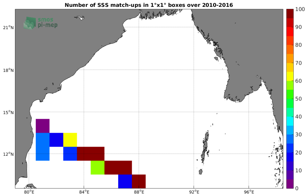
Figure 4: Number of SSS match-ups between TSG-LEGOS-DM SSS and the SMOS-L2-DPGS-v662 SSS product for the Bay of Bengal Pi-MEP region over 1^\circ \times 1^\circ boxes and for the full satellite product period.
