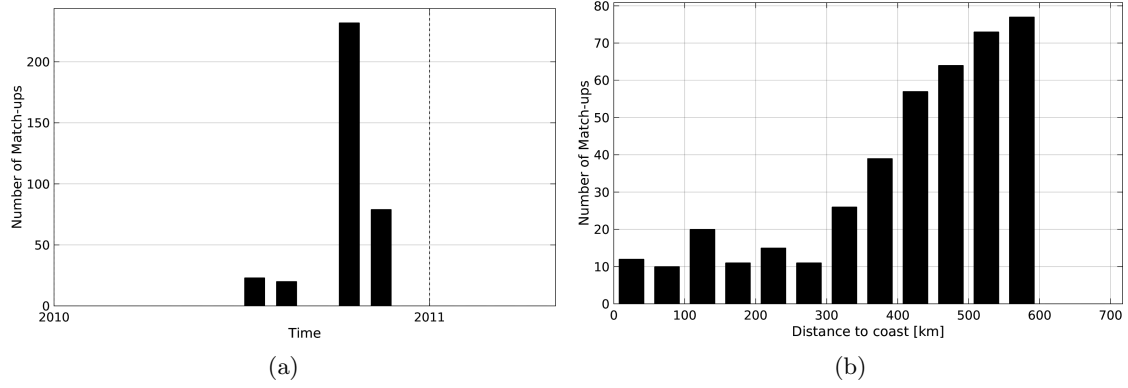
Figure 1: Number of match-ups between TSG-LEGOS-DM and SMOS-L2-DPGS-v662 SSS as a function of time (a) and as function of the distance to coast (b) over the Bay of Bengal Pi-MEP region and for the full satellite product period.
