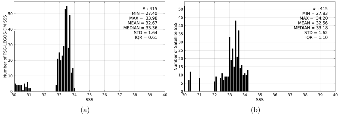
Figure 2: Histograms of SSS from TSG-LEGOS-DM (a) and SMOS-L2-DPGS-v662 (b) considering all match-up pairs per bins of 0.1 over the Bay of Bengal Pi-MEP region and for the full satellite product period.
