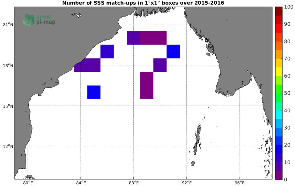
Figure 3: Number of SSS match-ups between Surface drifters SSS and the SMOS SSS L2 v662 (ESA) SSS product for the Bay of Bengal Pi-MEP region over 1^\circ \times 1^\circ boxes and for the full satellite product period.
