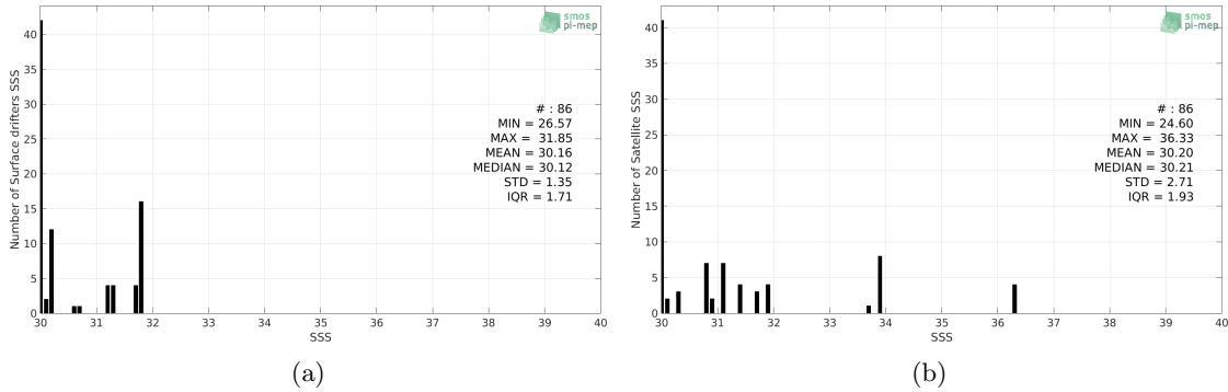
Figure 2: Histograms of SSS from Surface drifters (a) and SMOS SSS L2 v662 (ESA) (b) considering all match-up pairs per bins of 0.1 over the Bay of Bengal Pi-MEP region and for the full satellite product period.
