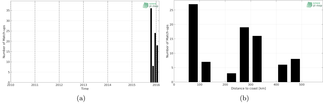
Figure 1: Number of match-ups between Surface drifters and SMOS SSS L2 v662 (ESA) SSS as a function of time (a) and as function of the distance to coast (b) over the Bay of Bengal Pi-MEP region and for the full satellite product period.
