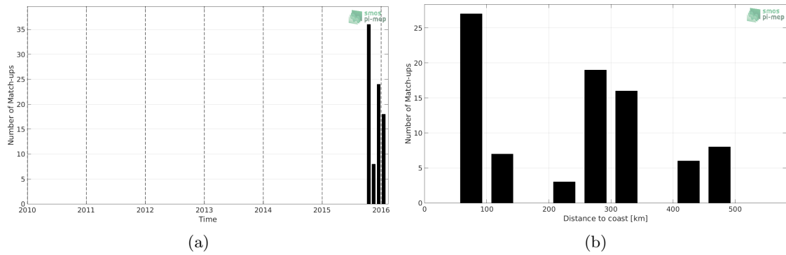
Figure 1: Number of match-ups between Surface drifters and SMOS SSS L2 v662 (ESA) SSS as a function of time (a) and as function of the distance to coast (b) over the Bay of Bengal Pi-MEP region and for the full satellite product period.
