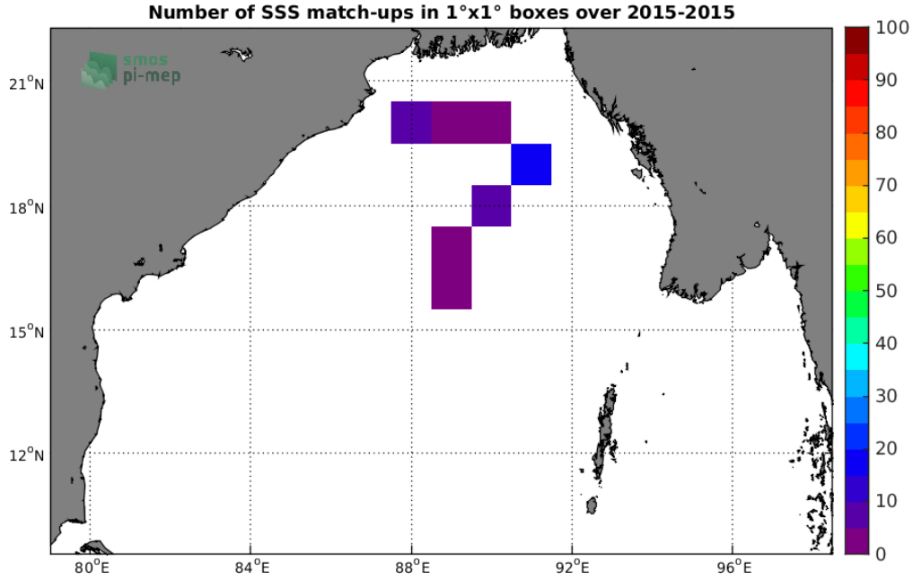
Figure 3: Number of SSS match-ups between Surface drifters SSS and the SMOS-L2-DPGS-v662 SSS product for the Bay of Bengal Pi-MEP region over 1^\circ \times 1^\circ boxes and for the full satellite product period.
