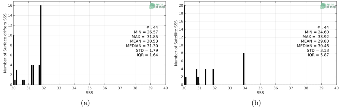
Figure 2: Histograms of SSS from Surface drifters (a) and SMOS-L2-DPGS-v662 (b) considering all match-up pairs per bins of 0.1 over the Bay of Bengal Pi-MEP region and for the full satellite product period.
