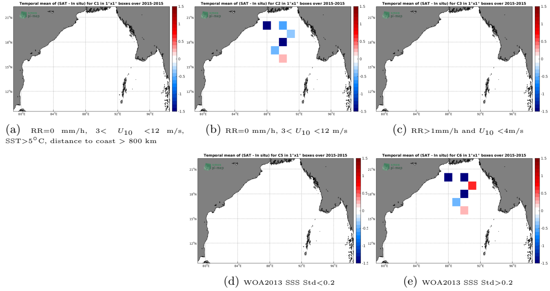
Figure 11: Temporal mean gridded over spatial boxes of size 1^\circ \times 1^\circ of \Delta SSS (SMOS-L2-DPGS-v662 - Surface drifters) for 5 different subdatasets corresponding to: RR=0 mm/h, 3 < U_{10} < 12 m/s, SST > 5^\circ C , distance to coast > 800 km (a), RR=0 mm/h, 3 < U_{10} < 12 m/s (b), RR > 1 mm/h and U_{10} < 4 m/s (c), WOA2013 SSS Std < 0.2 (d), WOA2013 SSS Std > 0.2 (e).
