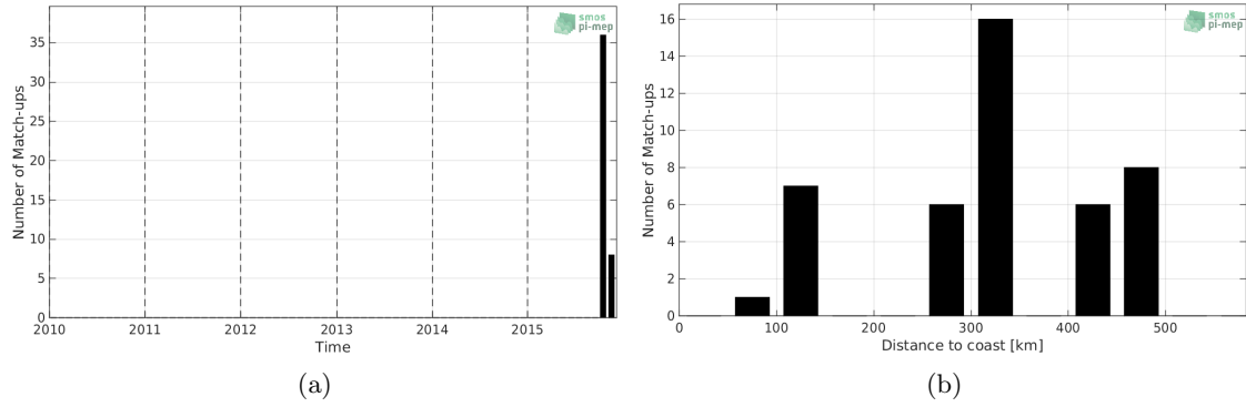
Figure 1: Number of match-ups between Surface drifters and SMOS-L2-DPGS-v662 SSS as a function of time (a) and as function of the distance to coast (b) over the Bay of Bengal Pi-MEP region and for the full satellite product period.
