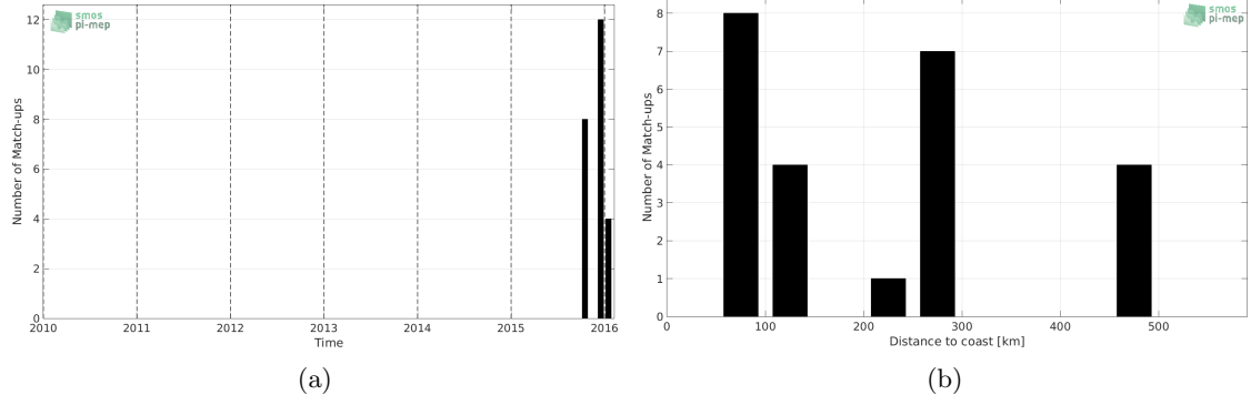
Figure 1: Number of match-ups between Surface drifters and SMOS-L2-DPGS-v662 SSS as a function of time (a) and as function of the distance to coast (b) over the Bay of Bengal Pi-MEP region and for the full satellite product period.
