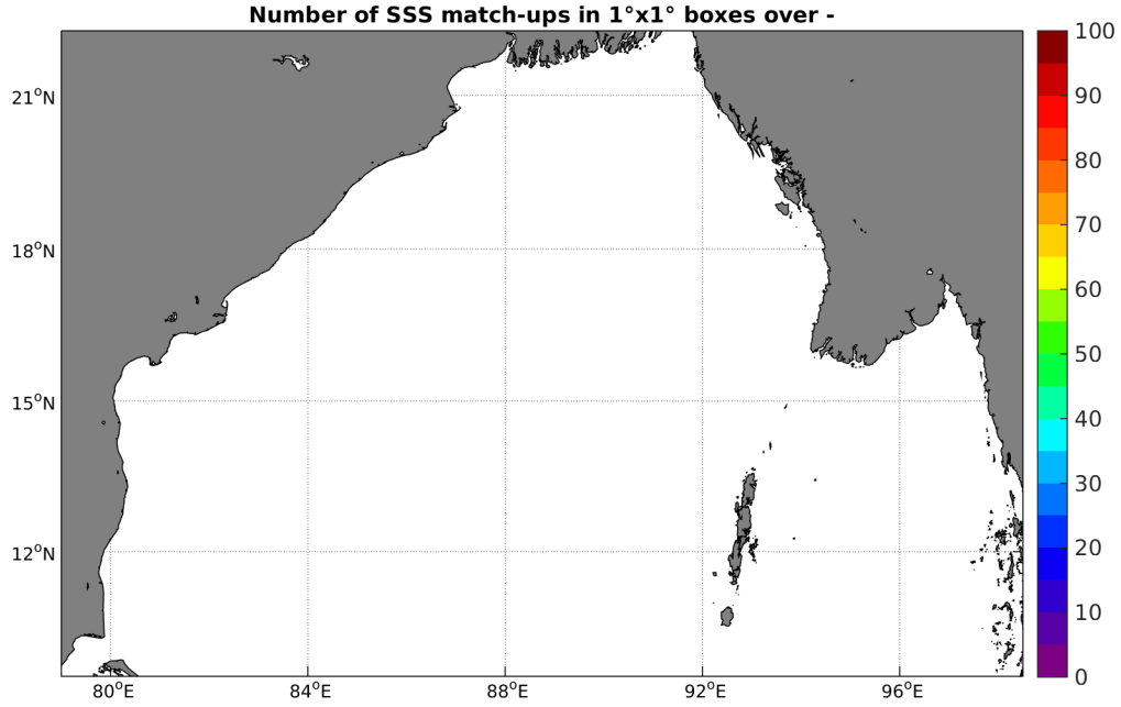
Figure 3: Number of SSS match-ups between Surface drifters SSS and the SMOS-L2-DPGS-v662 SSS product for the Bay of Bengal Pi-MEP region over 1°x1° boxes and for the full satellite product period.
