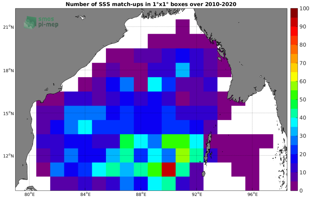
Figure 4: Number of SSS match-ups between Argo SSS and the SMOS SSS L2 v662 (ESA) SSS product for the Bay of Bengal Pi-MEP region over 1^\circ \times 1^\circ boxes and for the full satellite product period.
