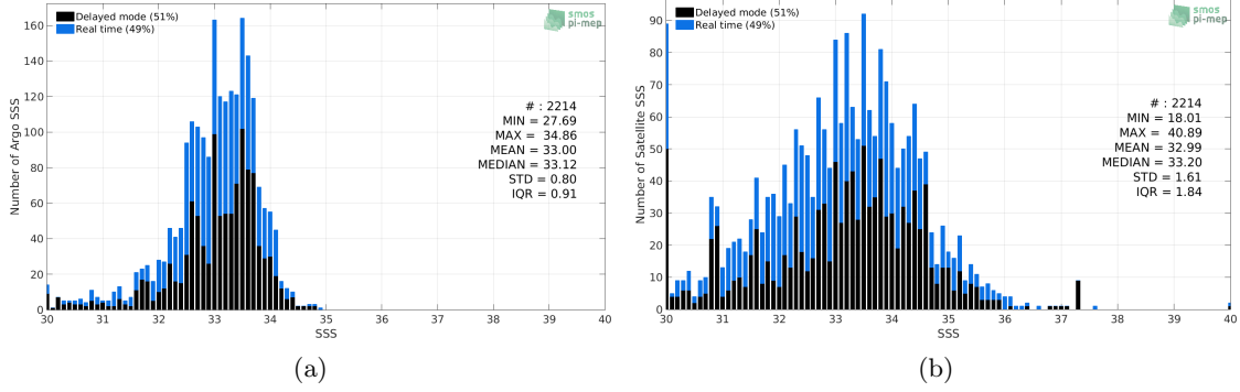
Figure 2: Histograms of SSS from Argo (a) and SMOS SSS L2 v662 (ESA) (b) considering all match-up pairs per bins of 0.1 over the Bay of Bengal Pi-MEP region and for the full satellite product period.
