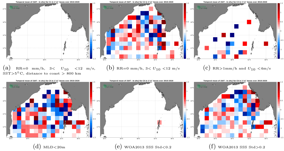
Figure 12: Temporal mean gridded over spatial boxes of size 1^\circ \times 1^\circ of \Delta SSS (SMOS SSS L2 v662 (ESA) - Argo) for 6 different subdatasets corresponding to: RR=0 mm/h, 3 < U_{10} < 12 m/s, SST > 5^\circ C , distance to coast > 800 km (a), RR=0 mm/h, 3 < U_{10} < 12 m/s (b), RR > 1 mm/h and U_{10} < 4 m/s (c), MLD < 20 m (d), WOA2013 SSS Std < 0.2 (e), WOA2013 SSS Std > 0.2 (f).
