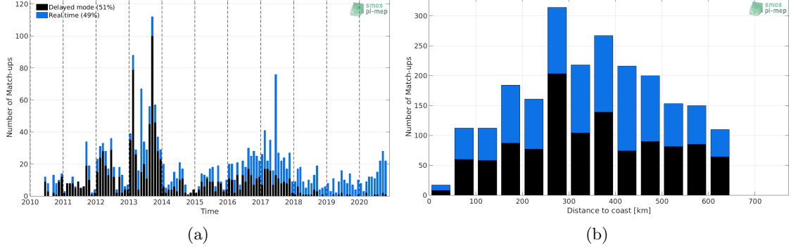
Figure 1: Number of match-ups between Argo and SMOS SSS L2 v662 (ESA) SSS as a function of time (a) and as function of the distance to coast (b) over the Bay of Bengal Pi-MEP region and for the full satellite product period.
